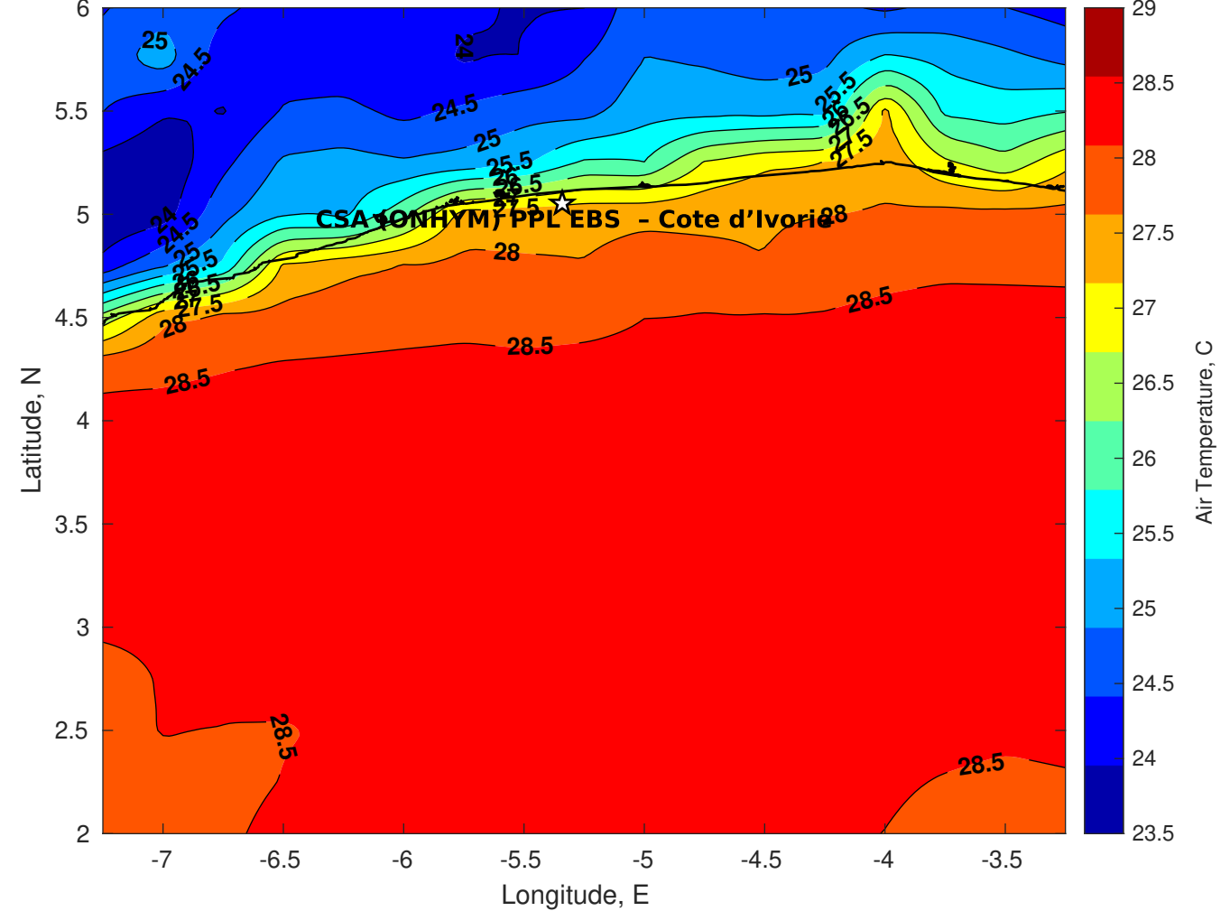
Air Temperature (C) for CSA (ONHYM) PPL EBS - Cote d'Ivoire at 02-Feb-2026
