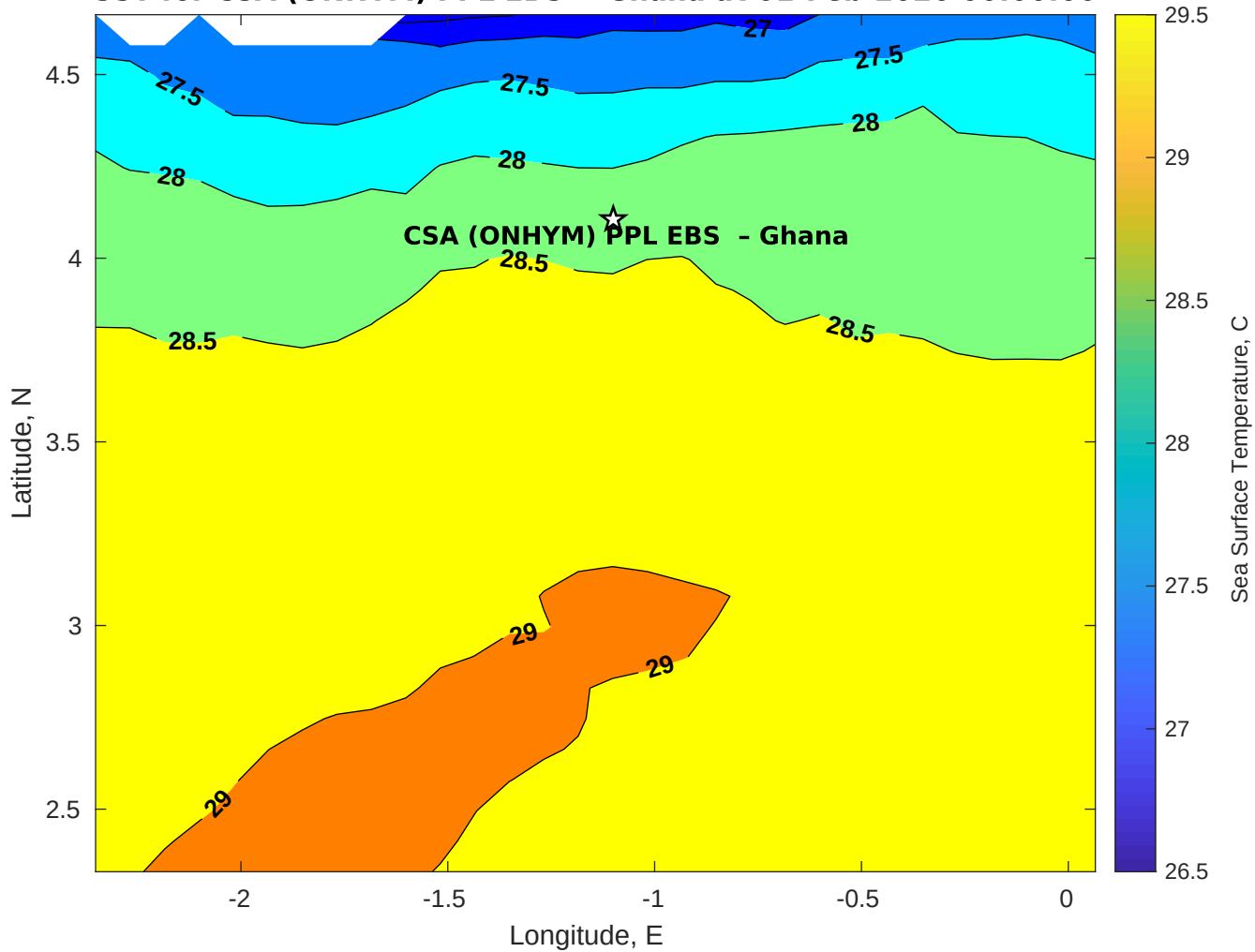
SST for CSA (ONHYM) PPL EBS - Ghana at 01-Feb-2026 00:00:00
