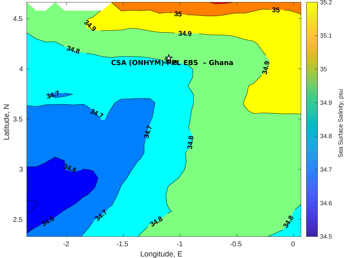
Surface Salinity for CSA (ONHYM) PPL EBS - Ghana at 01-Feb-2026 00:00:00
