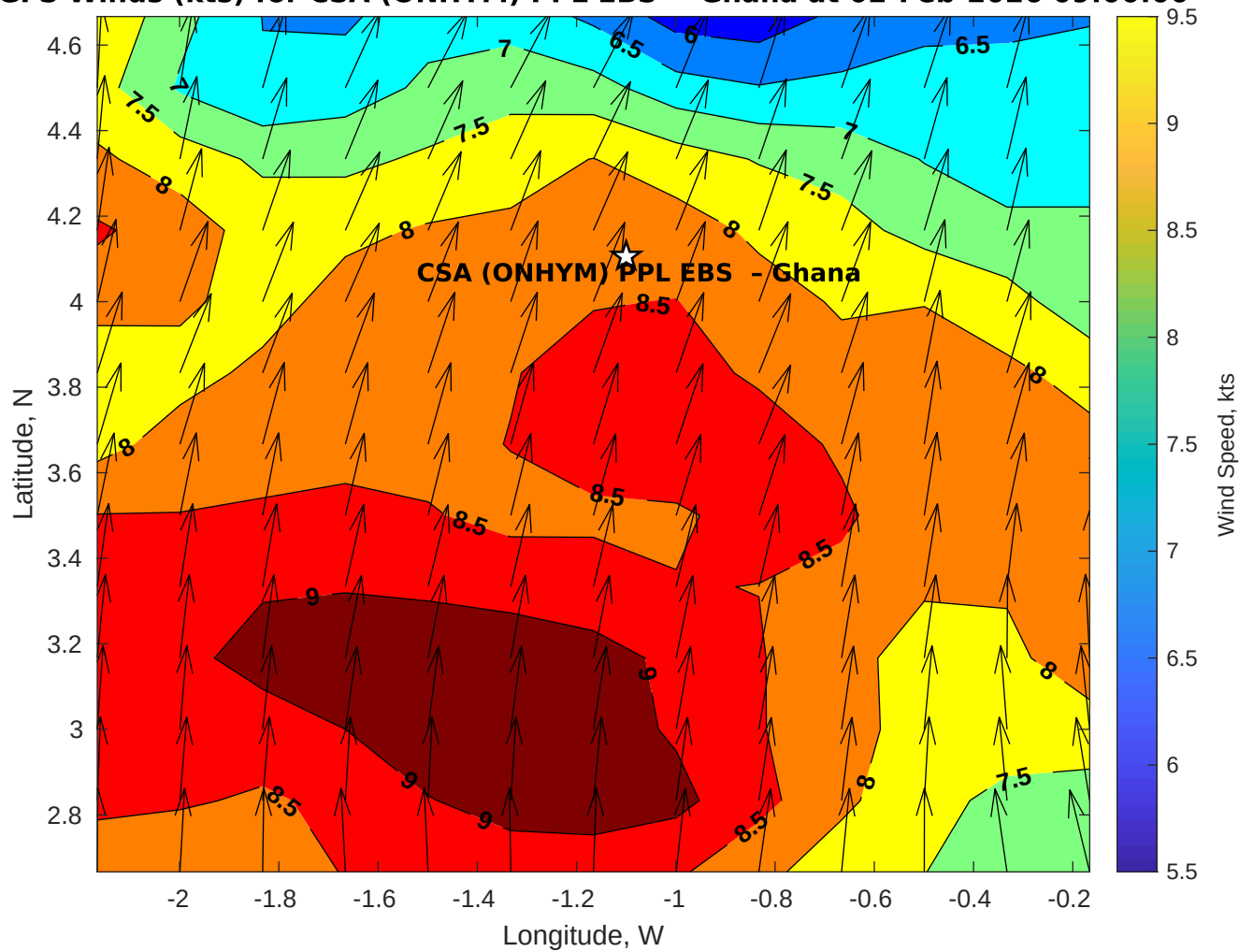
GFS Winds (kts) for CSA (ONHYM) PPL EBS - Ghana at 02-Feb-2026 09:00:00
