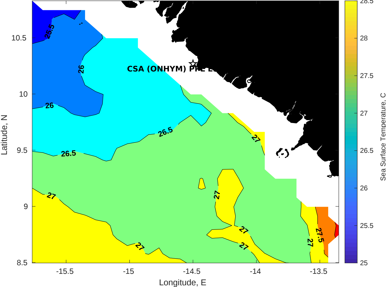
SST for CSA (ONHYM) PPL EBS - Guinea at 01-Feb-2026 00:00:00
