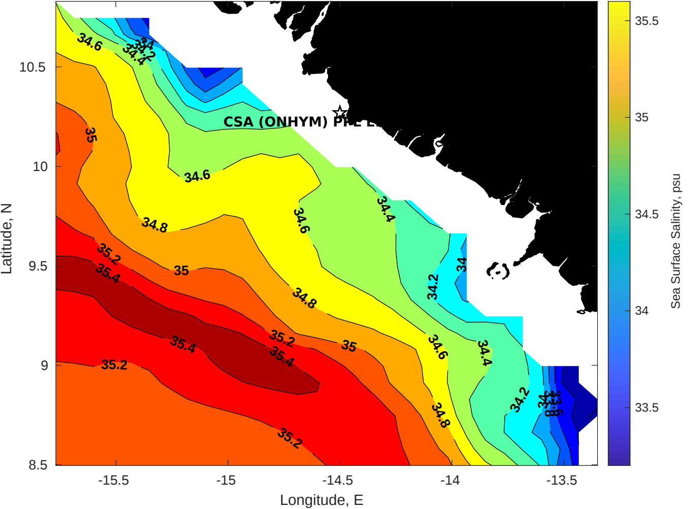
Surface Salinity for CSA (ONHYM) PPL EBS - Guinea at 01-Feb-2026 00:00:00
