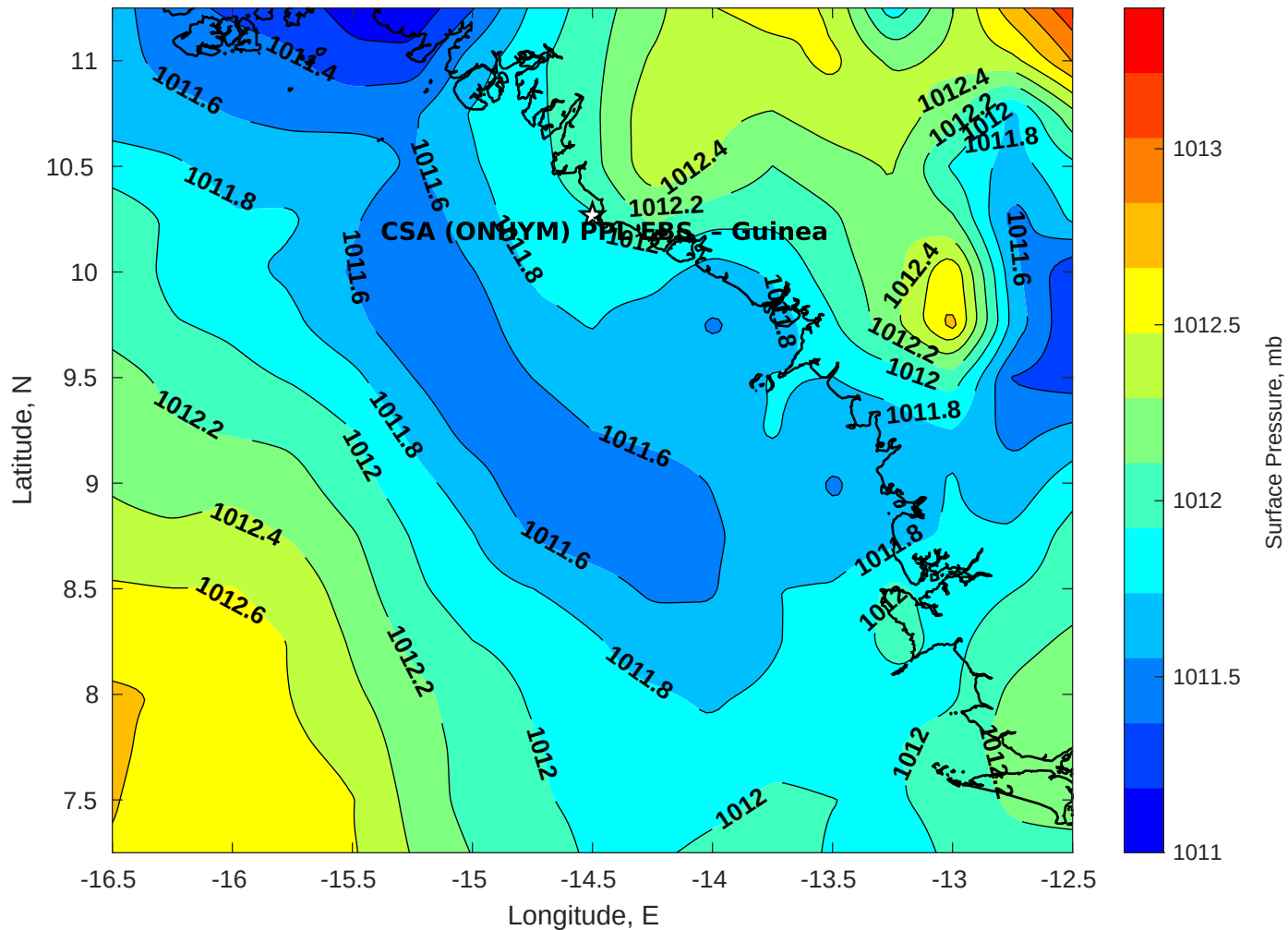
Surface Pressure (mb) for CSA (ONHYM) PPL EBS - Guinea at 03-Feb-2026 00:00:00
