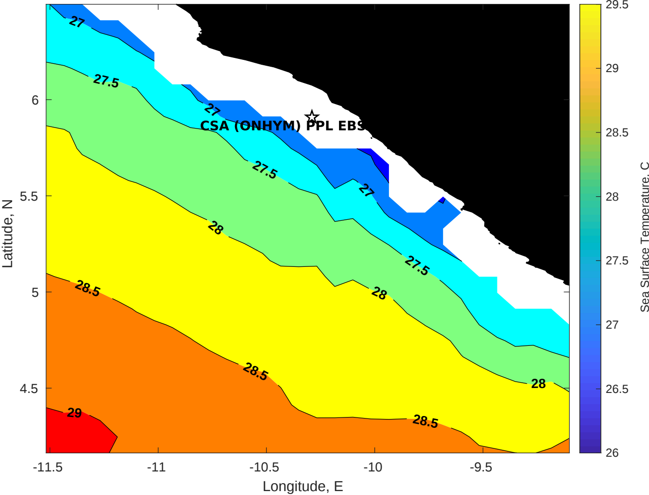
SST for CSA (ONHYM) PPL EBS - Liberia at 01-Feb-2026 00:00:00
