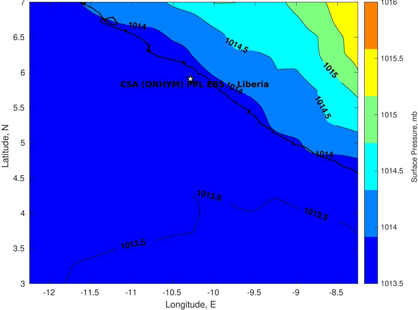
Surface Pressure (mb) for CSA (ONHYM) PPL EBS - Liberia at 04-Feb-2026 00:00:00
