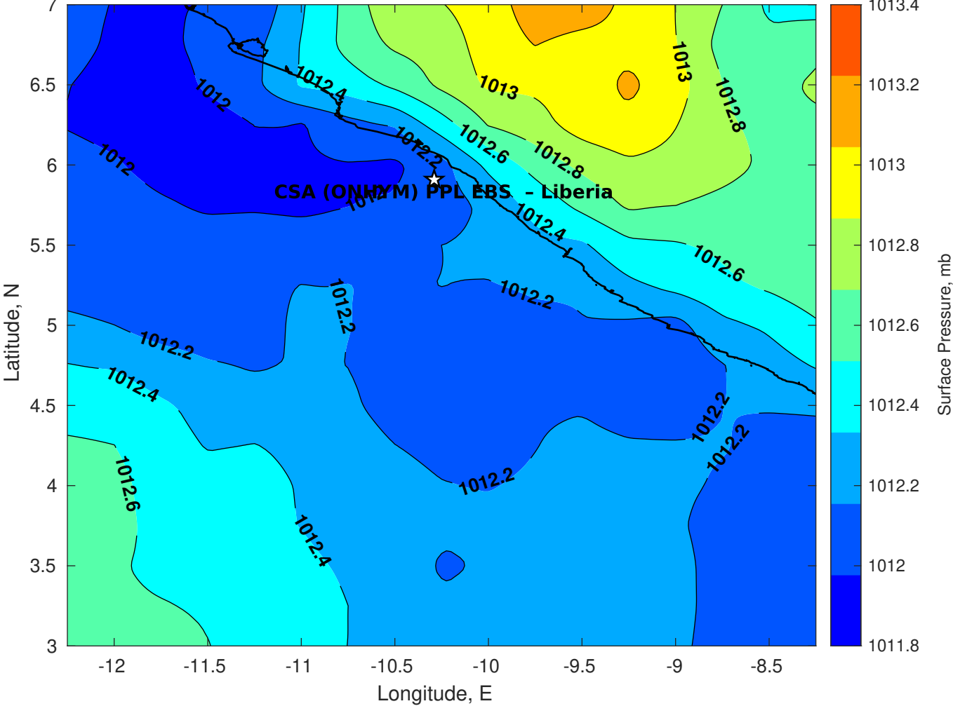
Surface Pressure (mb) for CSA (ONHYM) PPL EBS - Liberia at 03-Feb-2026 00:00:00
