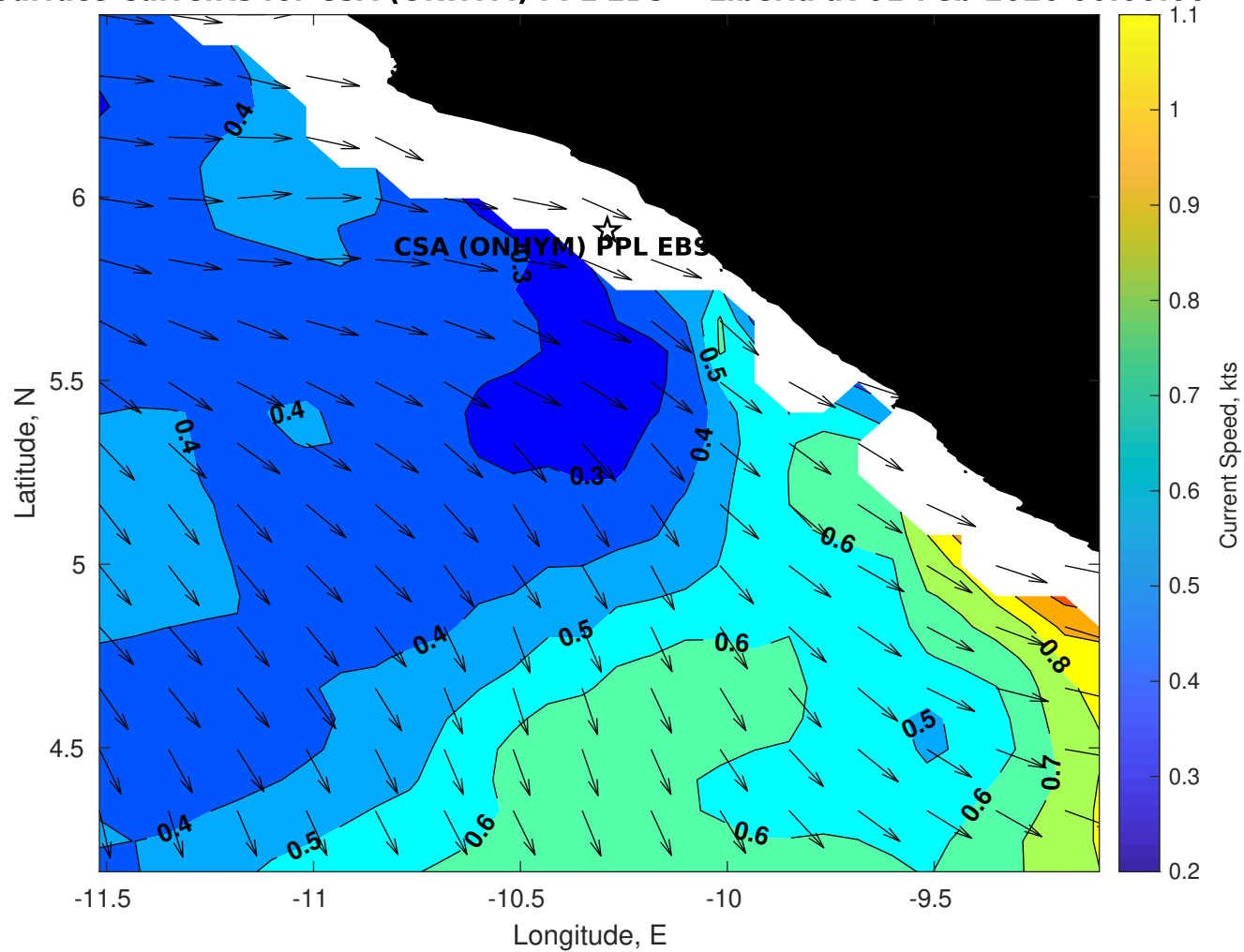
Surface Currents for CSA (ONHYM) PPL EBS - Liberia at 01-Feb-2026 00:00:00
