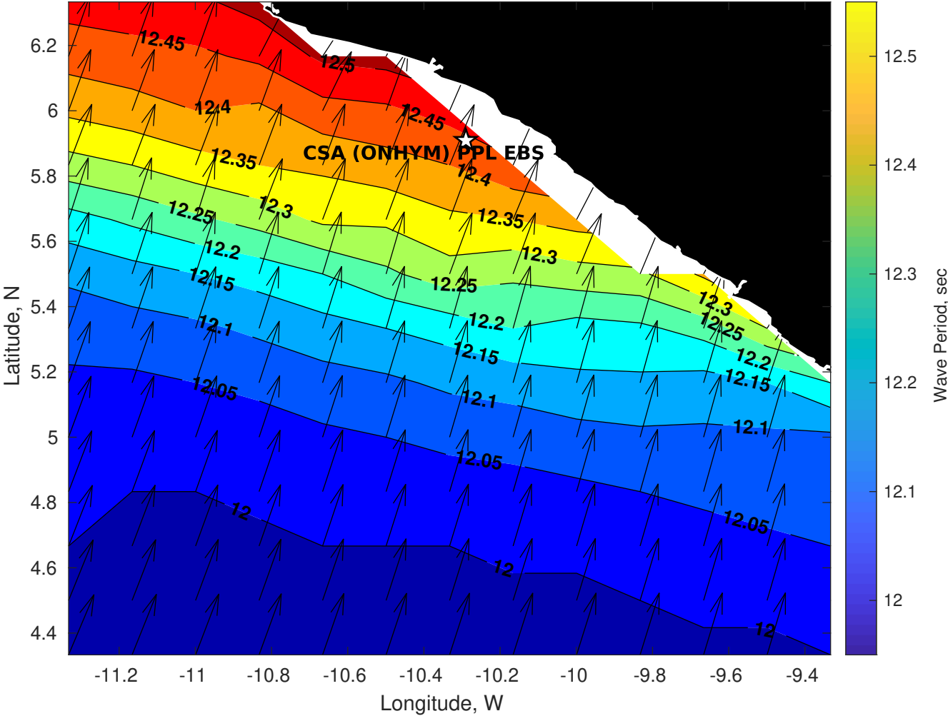
GFS Wave Period (sec) for CSA (ONHYM) PPL EBS - Liberia at 02-Feb-2026 09:00:00
