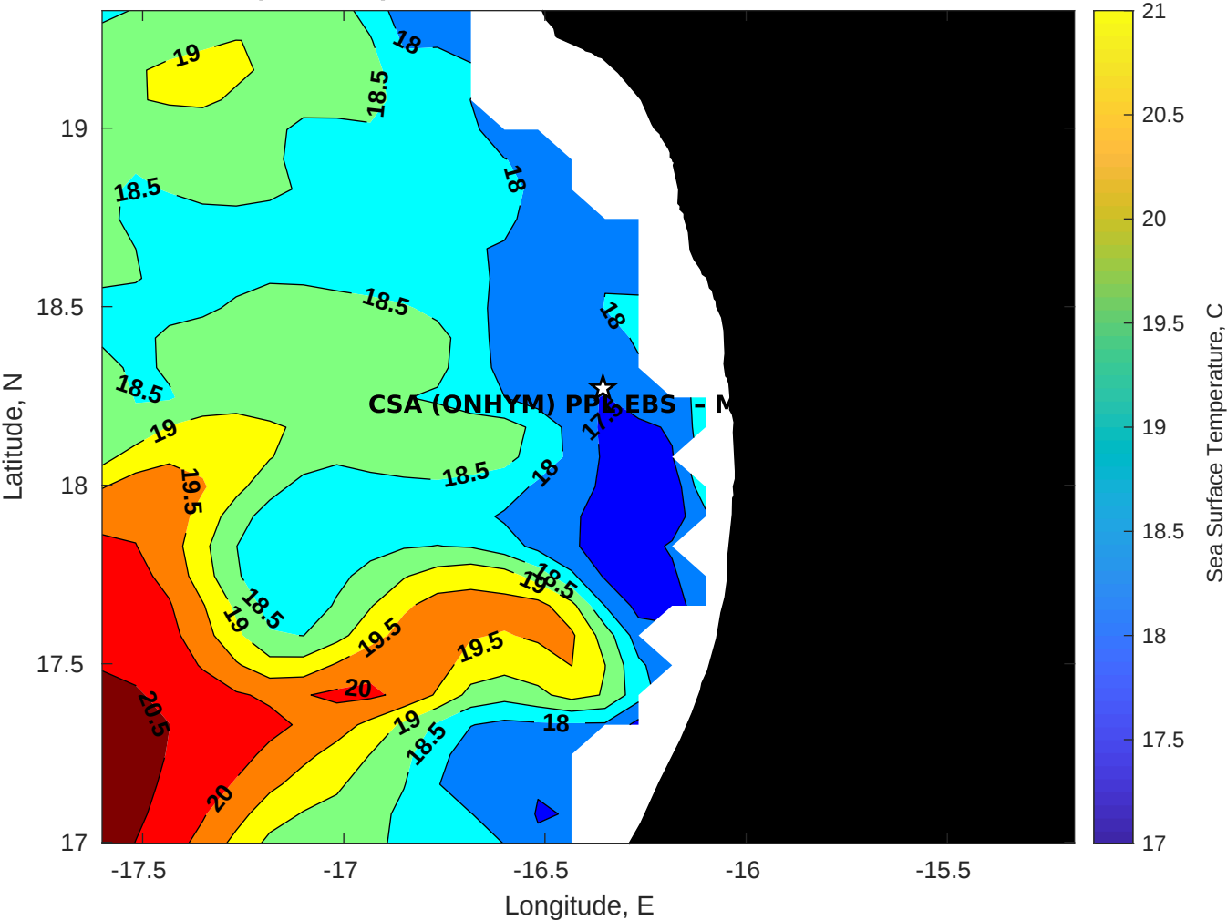
SST for CSA (ONHYM) PPL EBS - Mauritania at 01-Feb-2026 00:00:00
