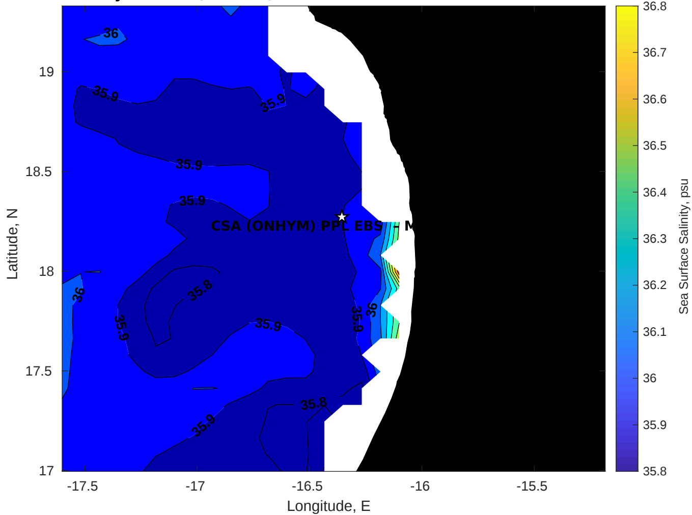
Surface Salinity for CSA (ONHYM) PPL EBS - Mauritania at 01-Feb-2026 00:00:00
