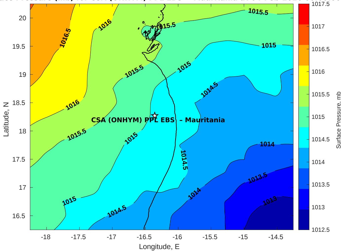
Surface Pressure (mb) for CSA (ONHYM) PPL EBS - Mauritania at 04-Feb-2026 00:00:00
