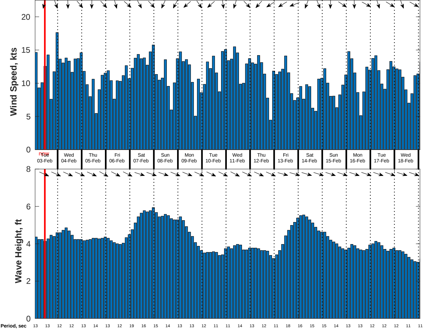
Wind & Wave Forecast for CSA (ONHYM) PPL EBS - Mauritania from 02-Feb-2026 01:00:00 to 18-Feb-2026 01:00:00
