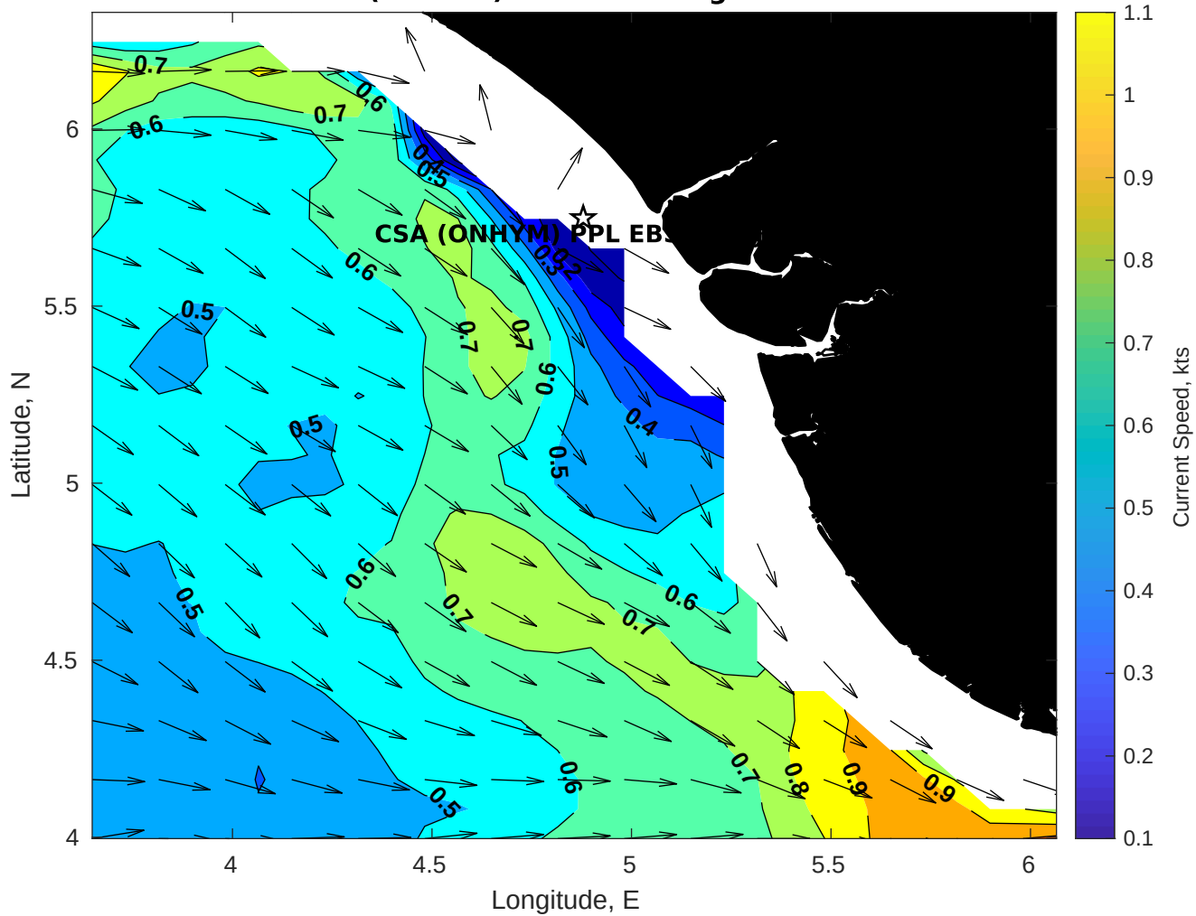
Surface Currents for CSA (ONHYM) PPL EBS - Nigeria at 01-Feb-2026 00:00:00
