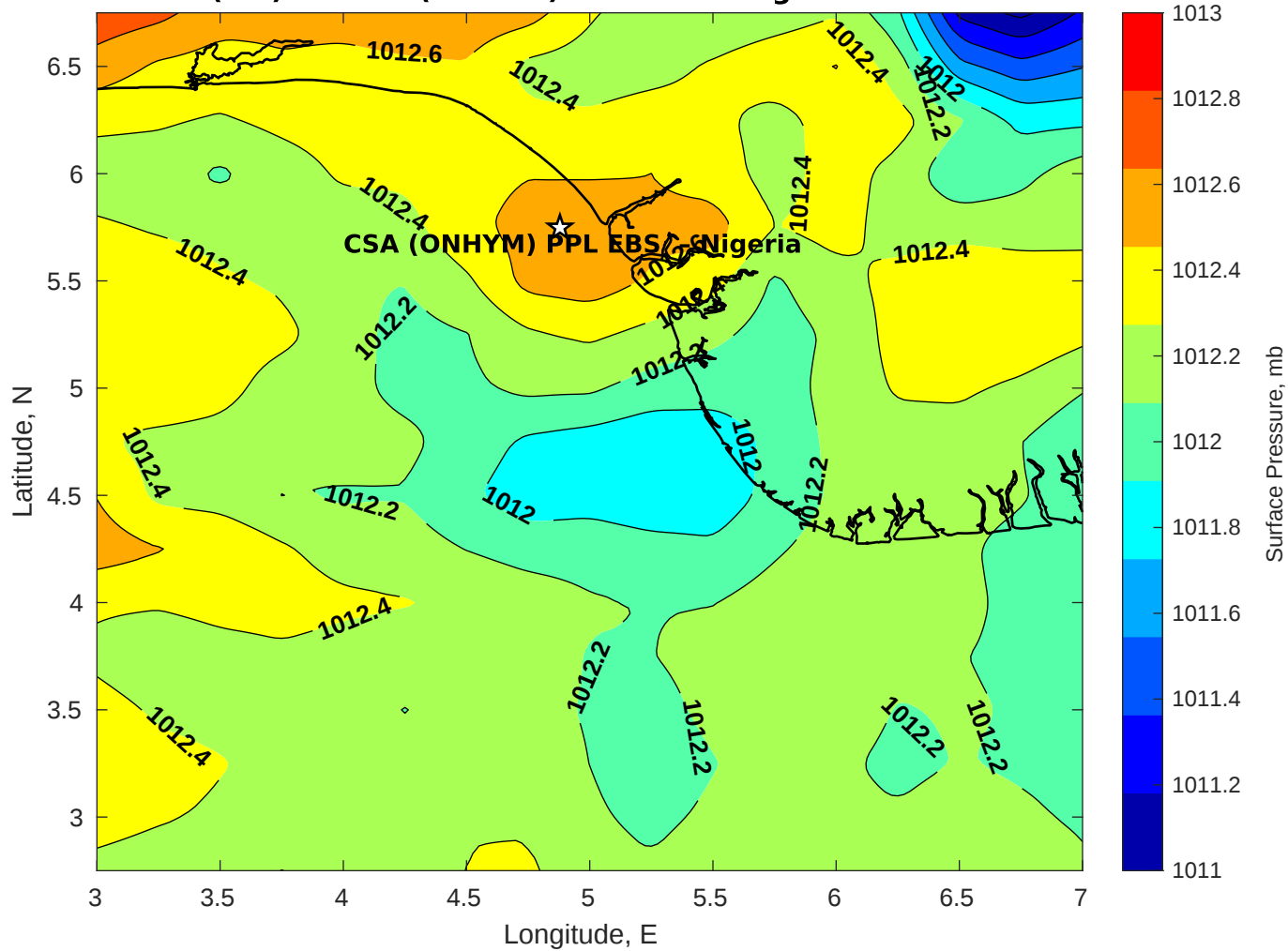
Surface Pressure (mb) for CSA (ONHYM) PPL EBS - Nigeria at 04-Feb-2026 00:00:00
