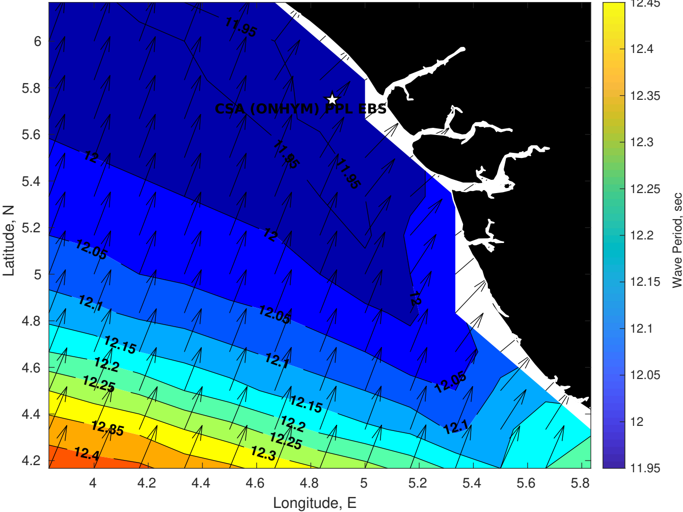
GFS Wave Period (sec) for CSA (ONHYM) PPL EBS - Nigeria at 02-Feb-2026 09:00:00
