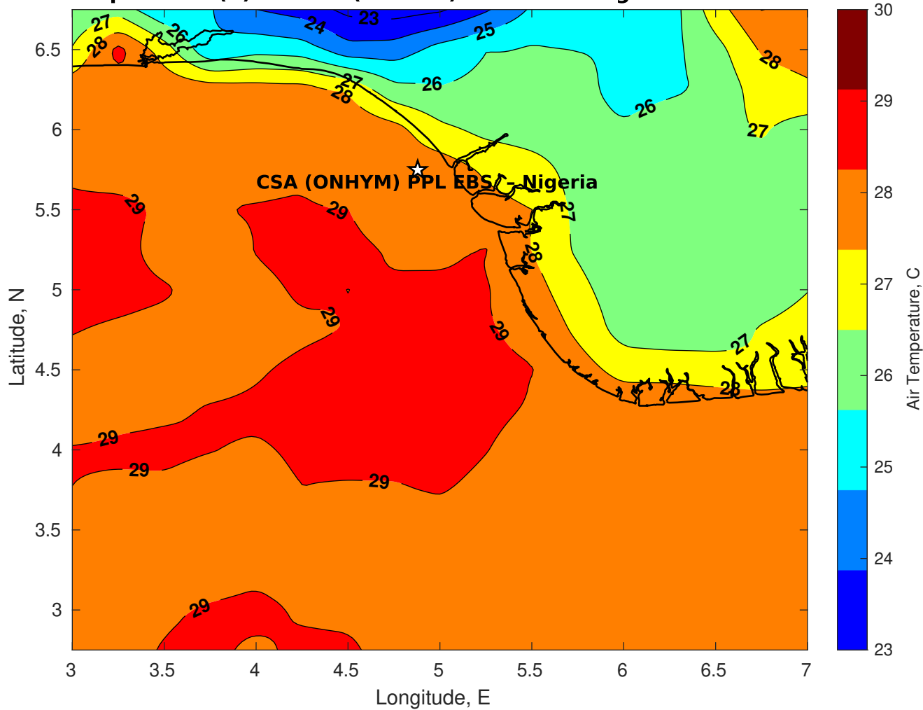
Air Temperature (C) for CSA (ONHYM) PPL EBS - Nigeria at 02-Feb-2026
