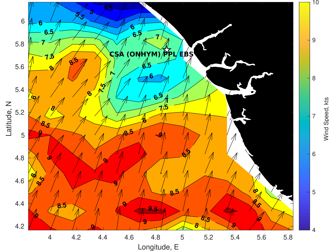
GFS Winds (kts) for CSA (ONHYM) PPL EBS - Nigeria at 02-Feb-2026 09:00:00
