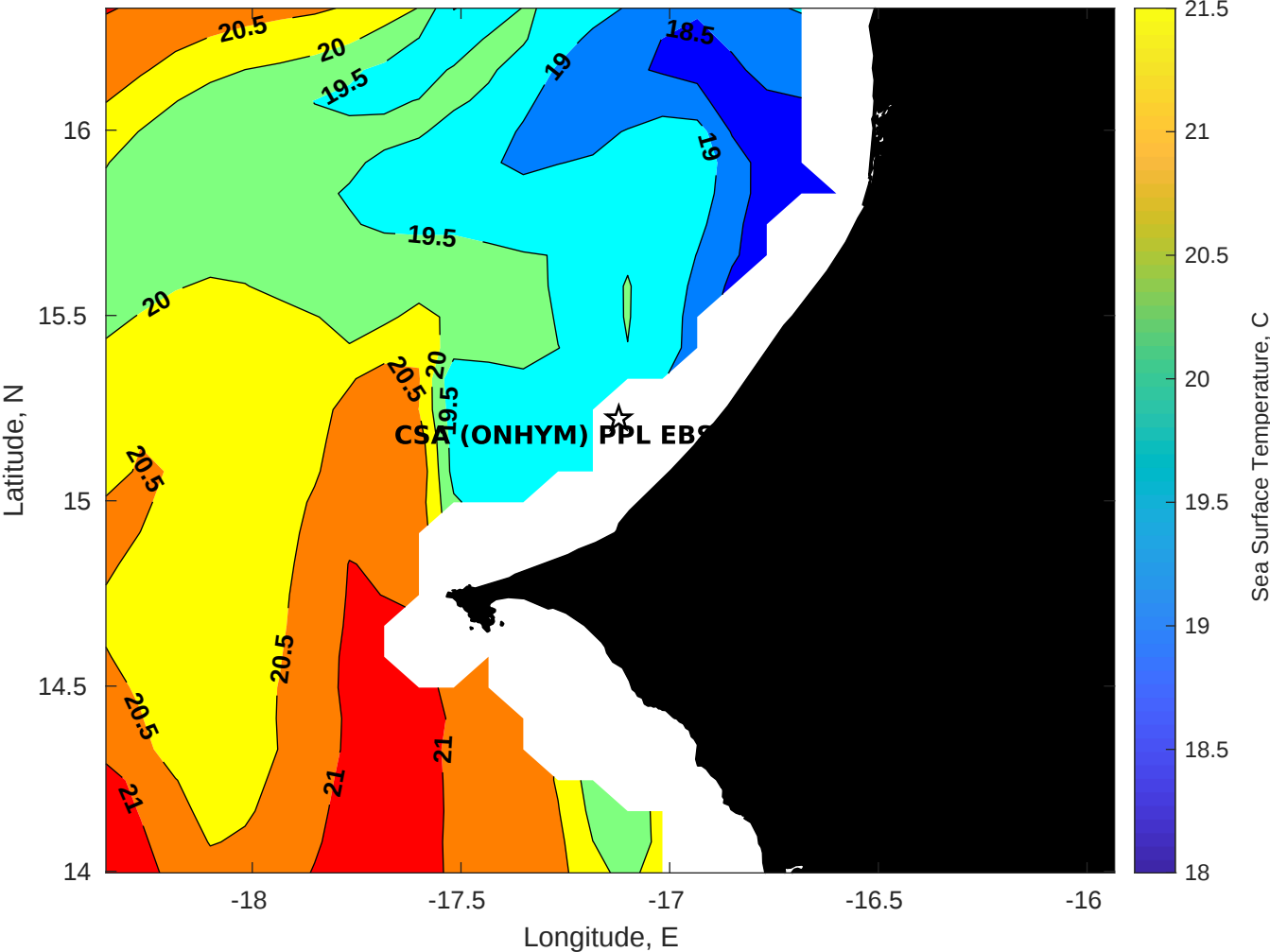
SST for CSA (ONHYM) PPL EBS - Senegal at 01-Feb-2026 00:00:00
