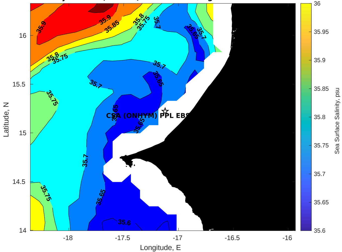
Surface Salinity for CSA (ONHYM) PPL EBS - Senegal at 01-Feb-2026 00:00:00
