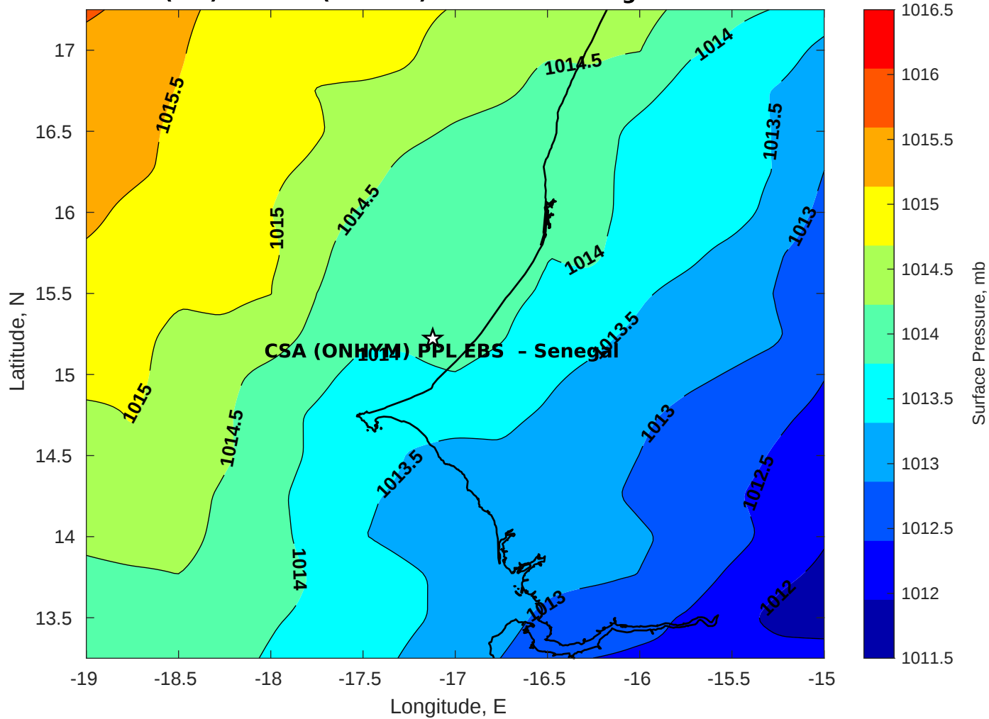
Surface Pressure (mb) for CSA (ONHYM) PPL EBS - Senegal at 04-Feb-2026 00:00:00
