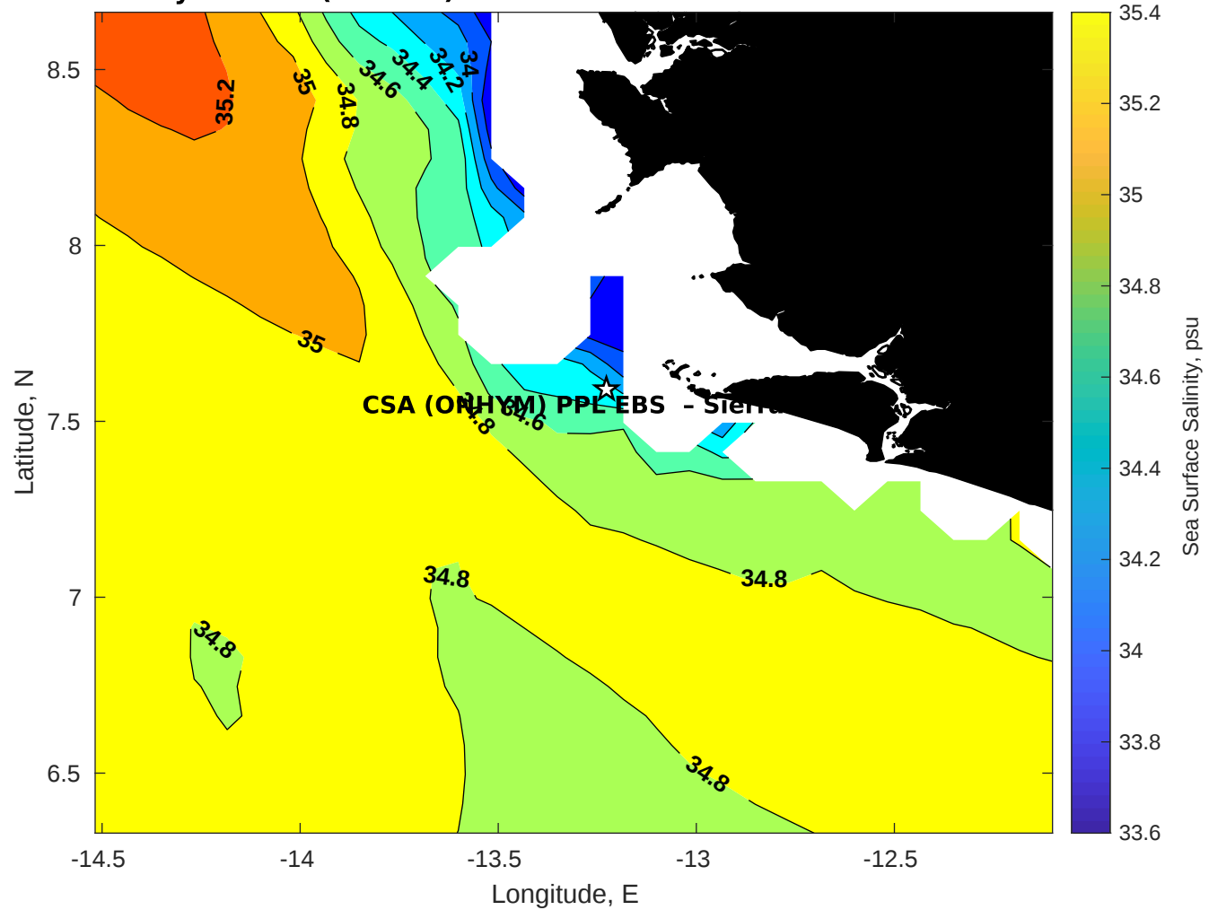
Surface Salinity for CSA (ONHYM) PPL EBS - Sierra Leone at 01-Feb-2026 00:00:00
