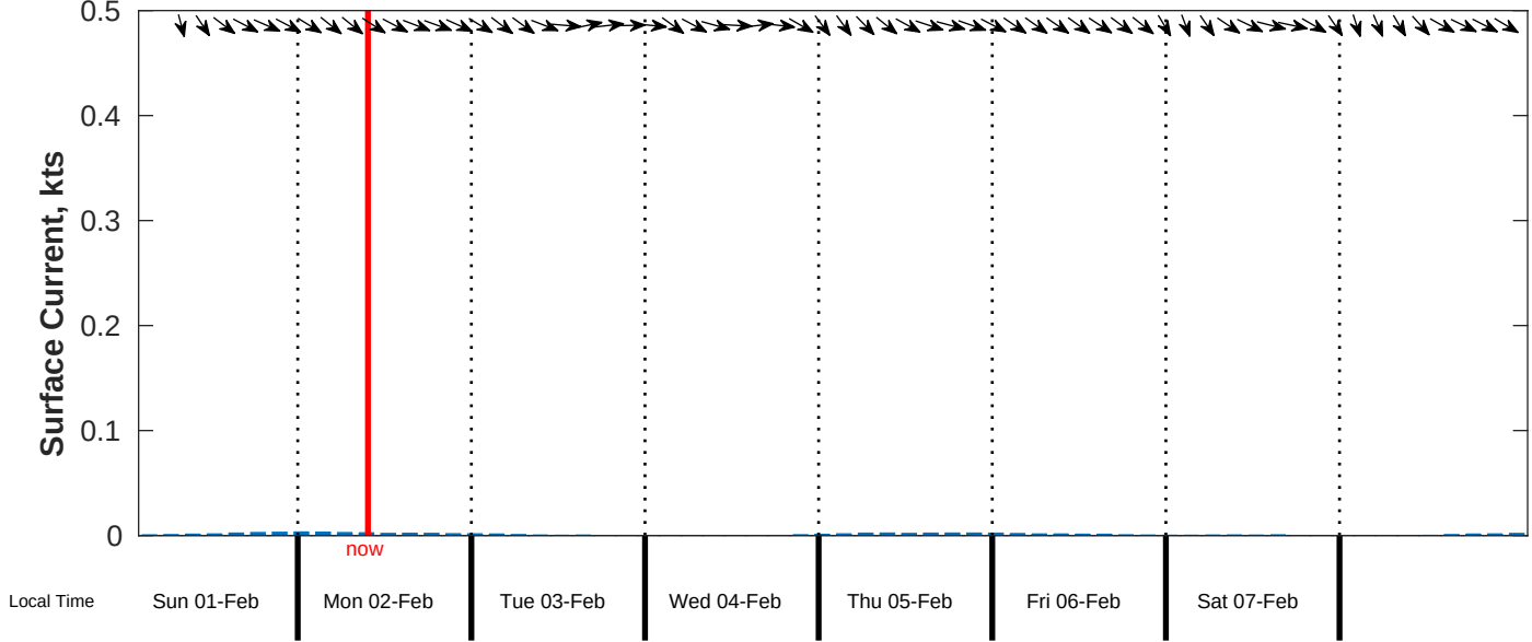
Surface Current Forecast for CSA (ONHYM) PPL EBS - Sierra Leone from 01-Feb-2026 00:00:00 to 09-Feb-2026 00:00:00
