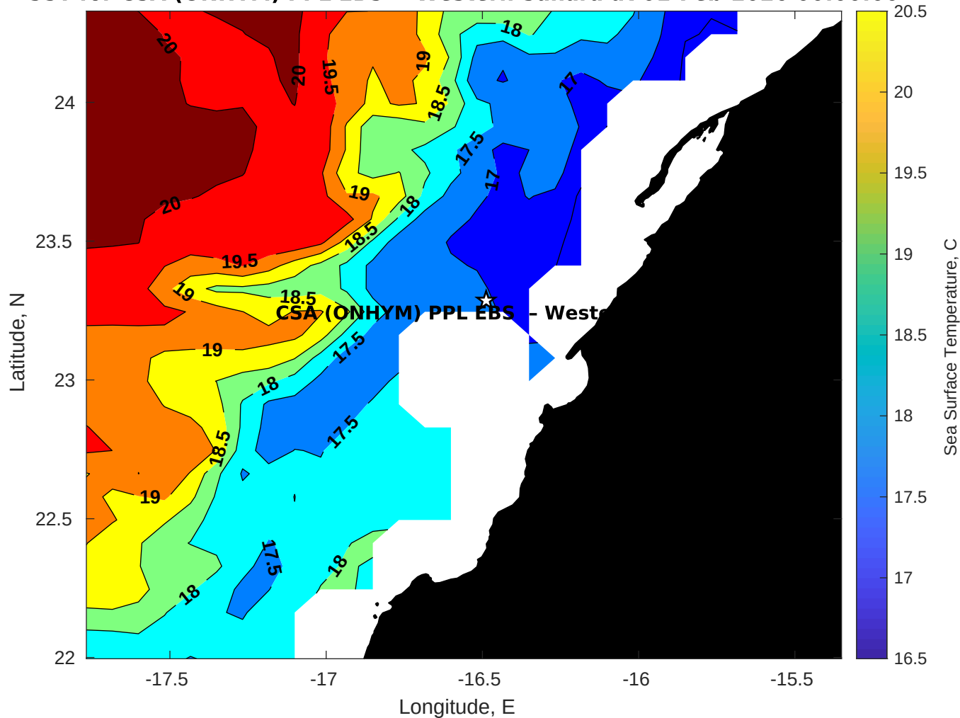
SST for CSA (ONHYM) PPL EBS - Western Sahara at 01-Feb-2026 00:00:00
