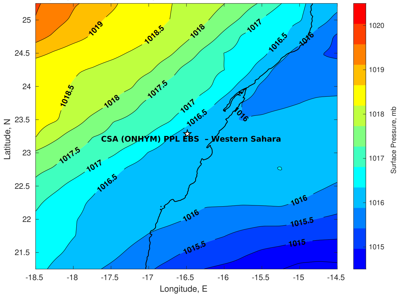
Surface Pressure (mb) for CSA (ONHYM) PPL EBS - Western Sahara at 02-Feb-2026 00:00:00
