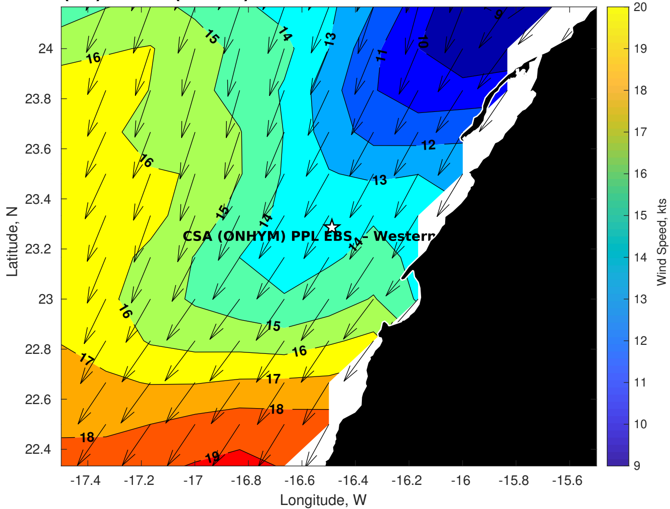
GFS Winds (kts) for CSA (ONHYM) PPL EBS - Western Sahara at 02-Feb-2026 09:00:00
