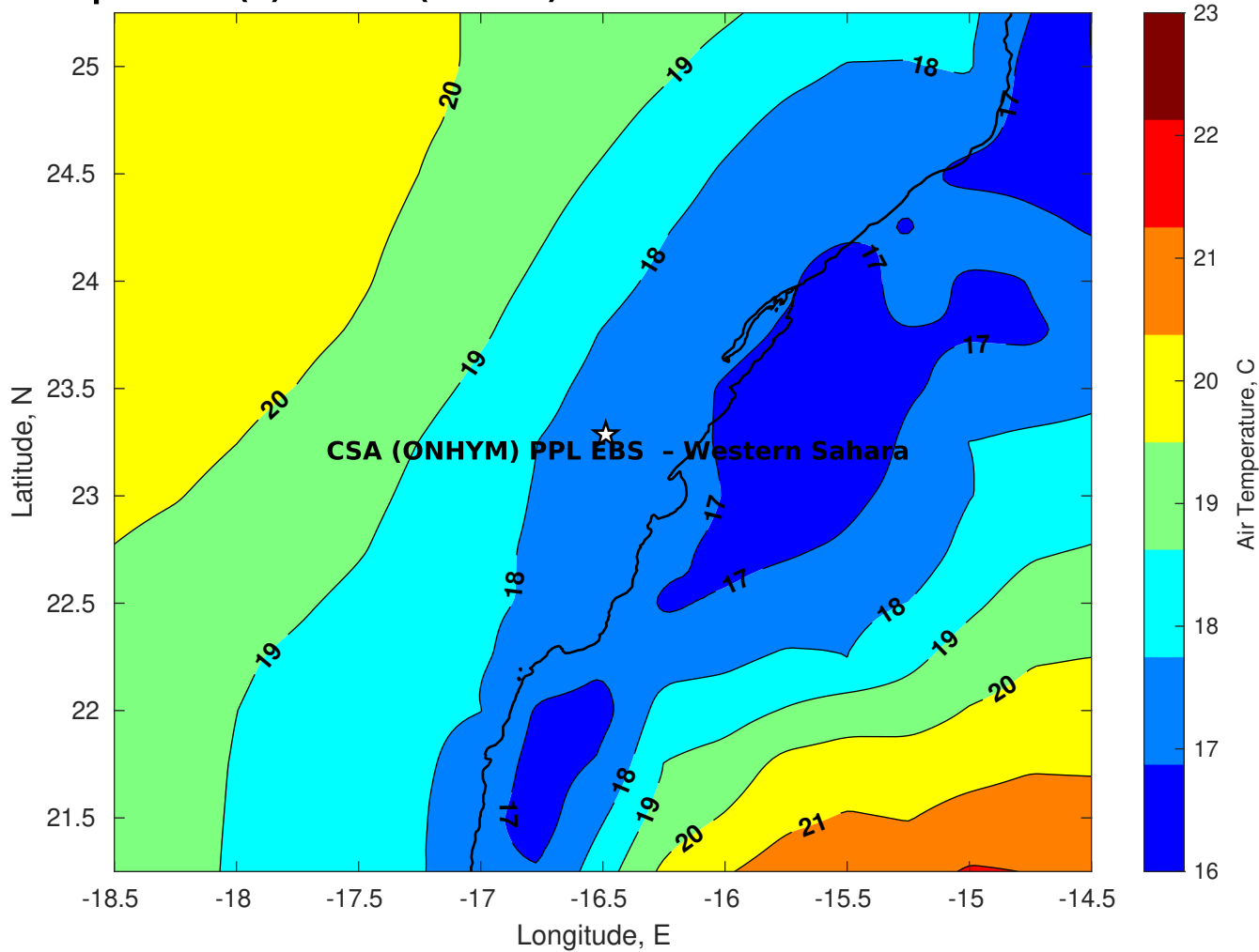
Air Temperature (C) for CSA (ONHYM) PPL EBS - Western Sahara at 02-Feb-2026
