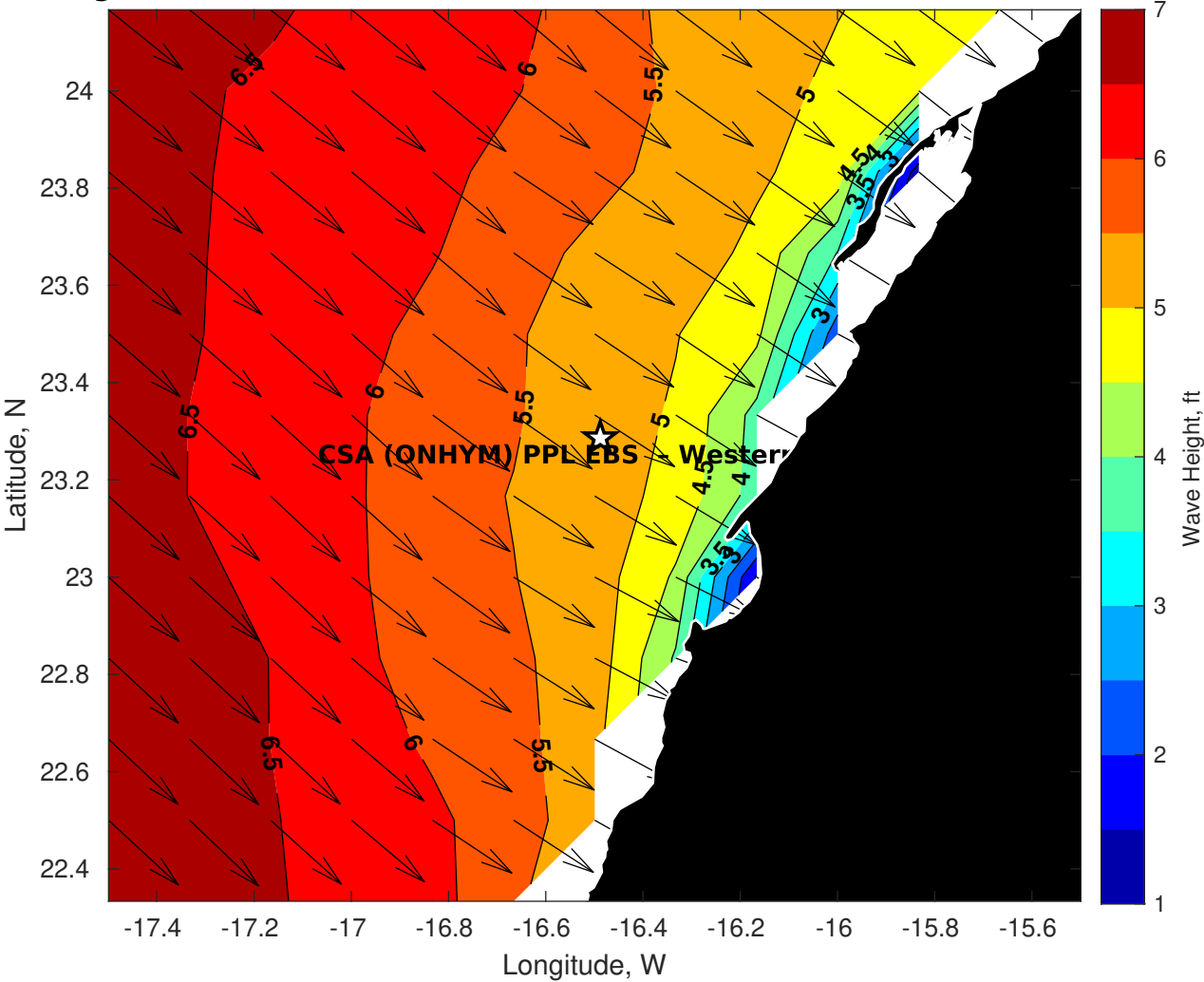
GFS Wave Height (ft) for CSA (ONHYM) PPL EBS - Western Sahara at 02-Feb-2026 09:00:00
