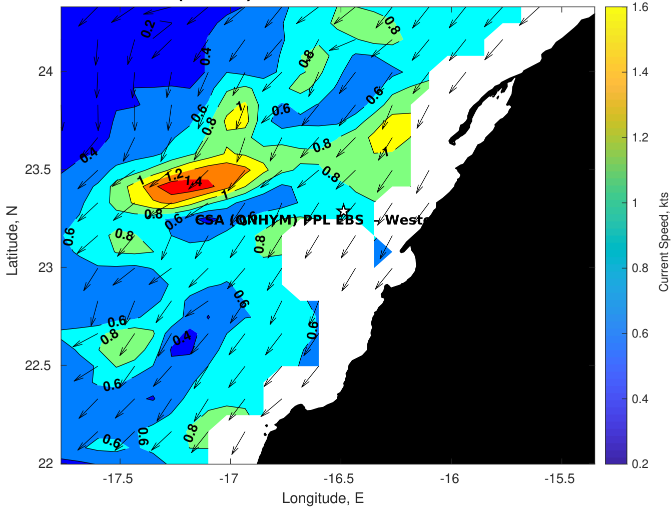
Surface Currents for CSA (ONHYM) PPL EBS - Western Sahara at 01-Feb-2026 00:00:00
