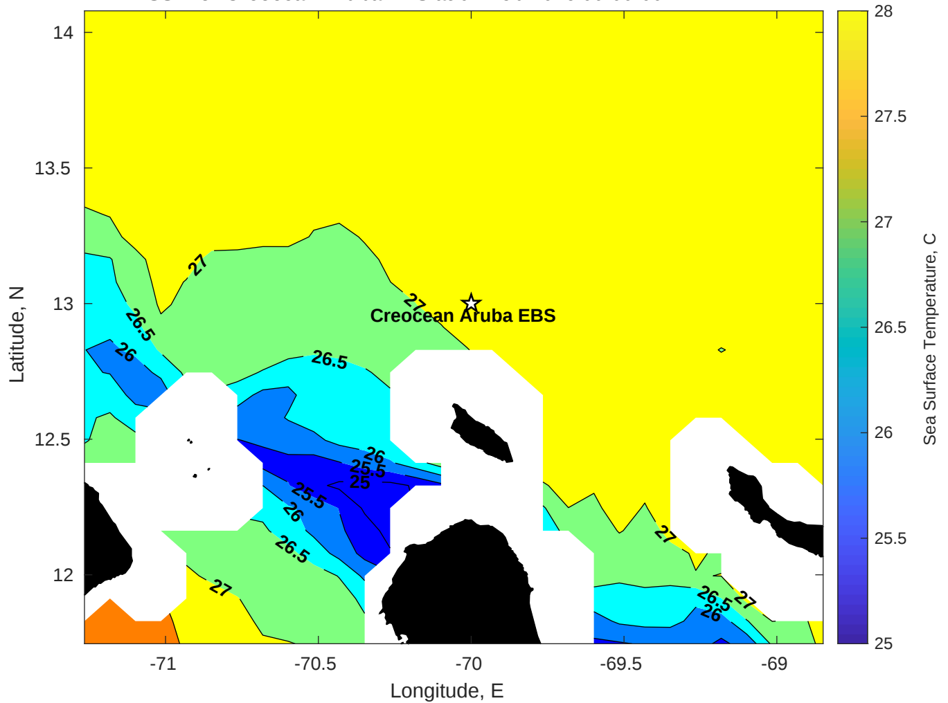
SST for Creolecean Aruba EBS at 01-Feb-2026 00:00:00
