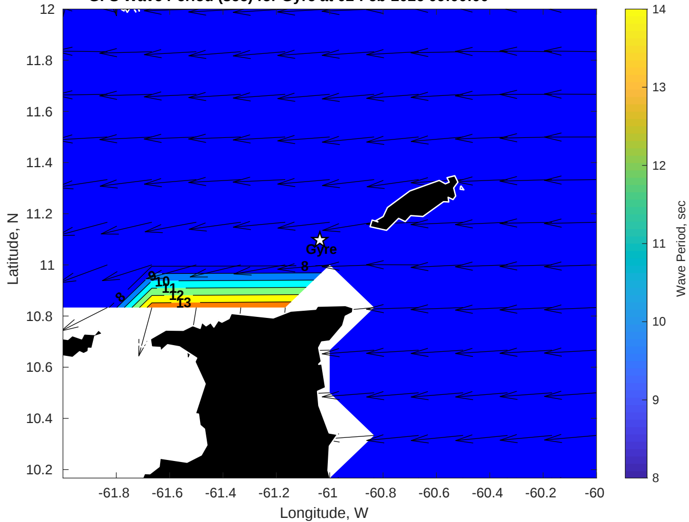
GFS Wave Period (sec) for Gyre at 02-Feb-2026 09:00:00
