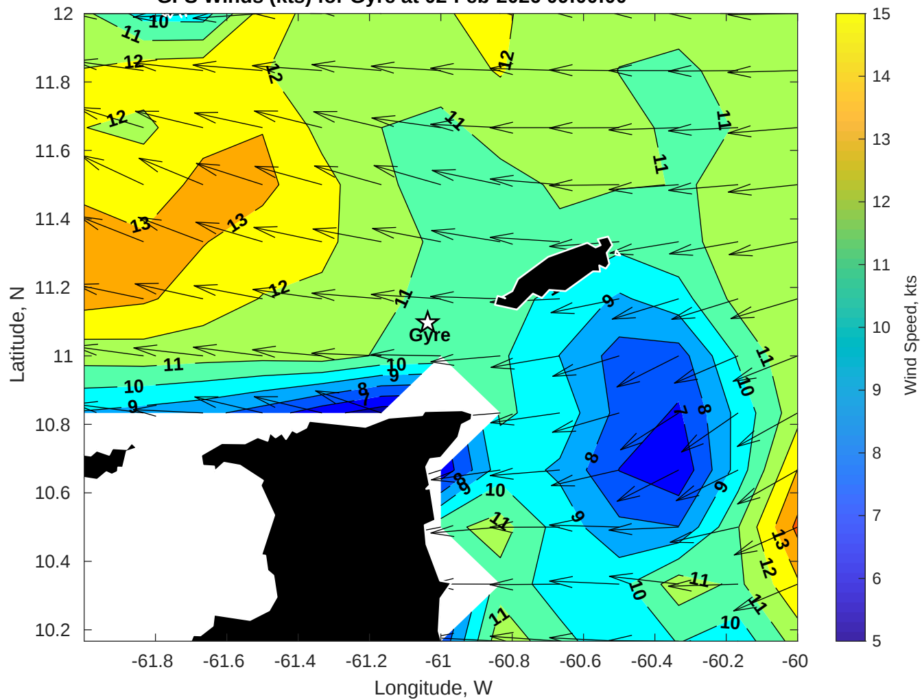
GFS Winds (kts) for Gyre at 02-Feb-2026 09:00:00
