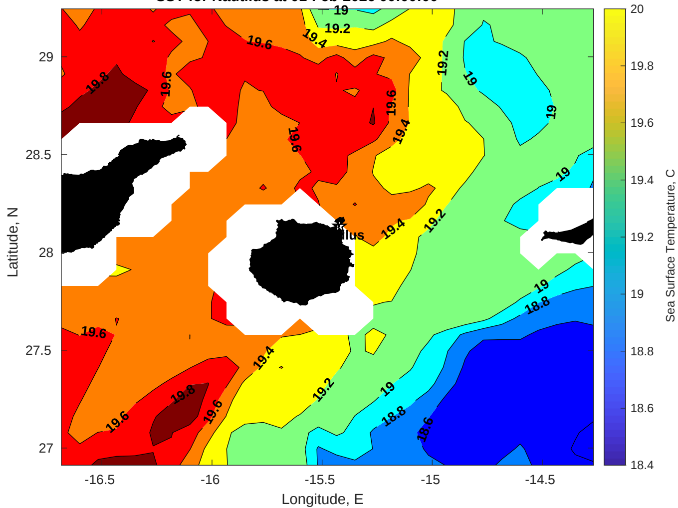
SST for Nautilus at 01-Feb-2026 00:00:00
