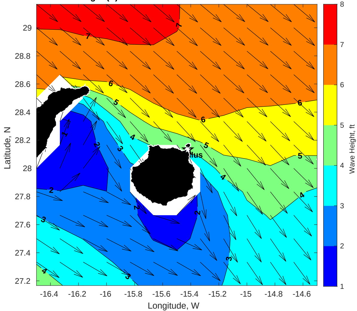
GFS Wave Height (ft) for Nautilus at 02-Feb-2026 09:00:00
