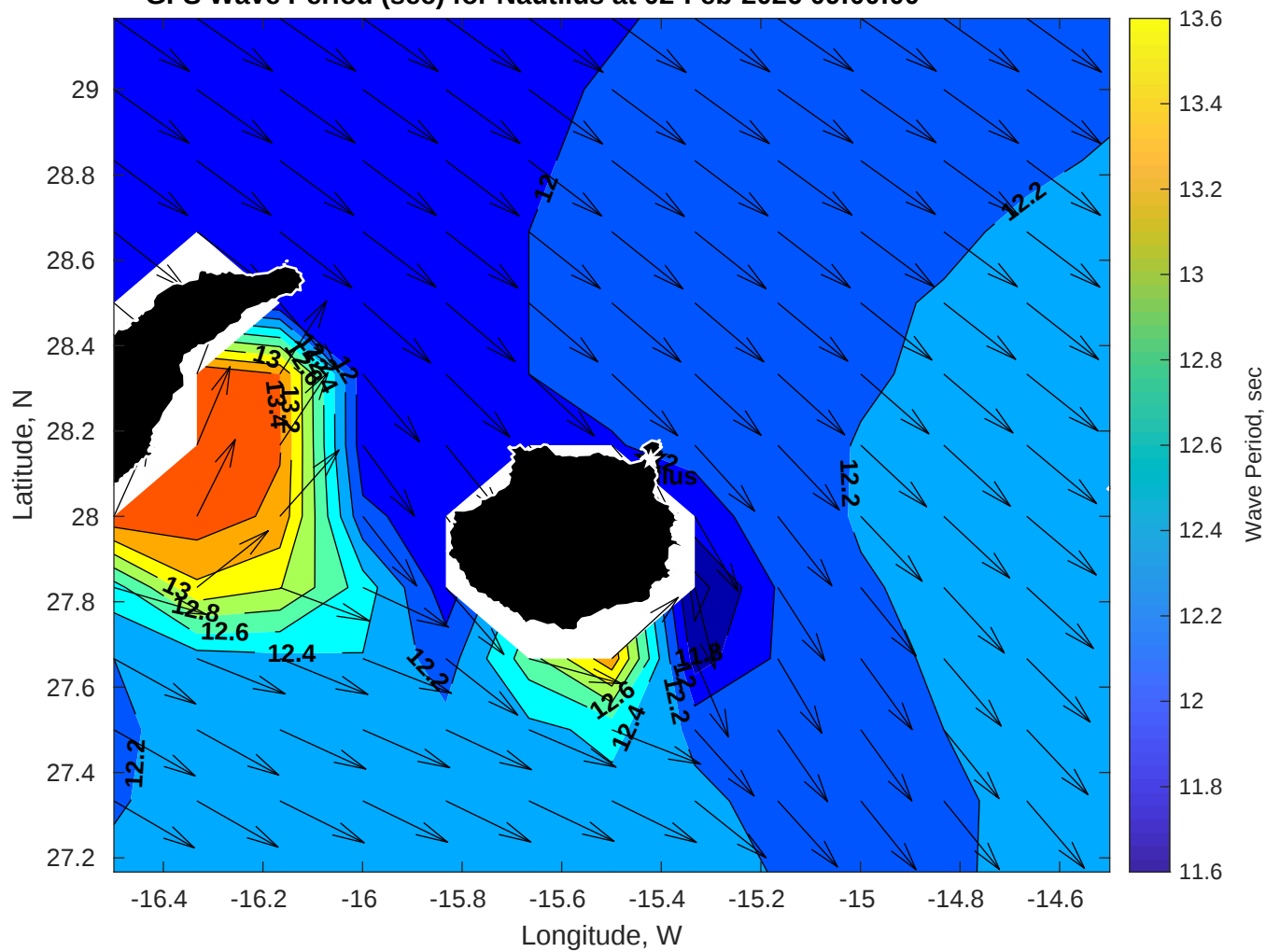
GFS Wave Period (sec) for Nautilus at 02-Feb-2026 09:00:00
