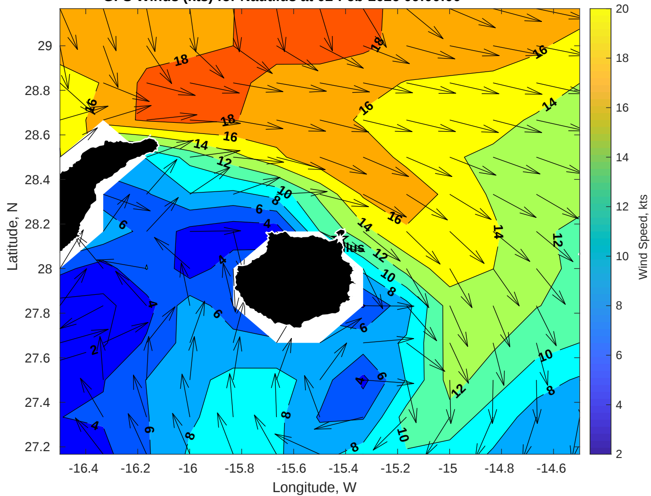
GFS Winds (kts) for Nautilus at 02-Feb-2026 09:00:00
