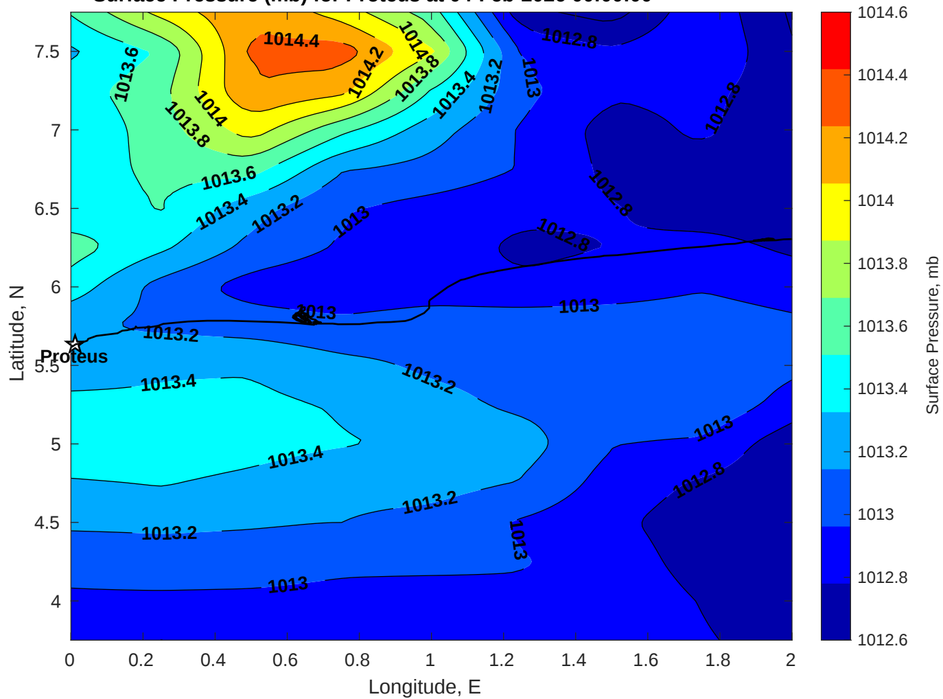
Surface Pressure (mb) for Proteus at 04-Feb-2026 00:00:00
