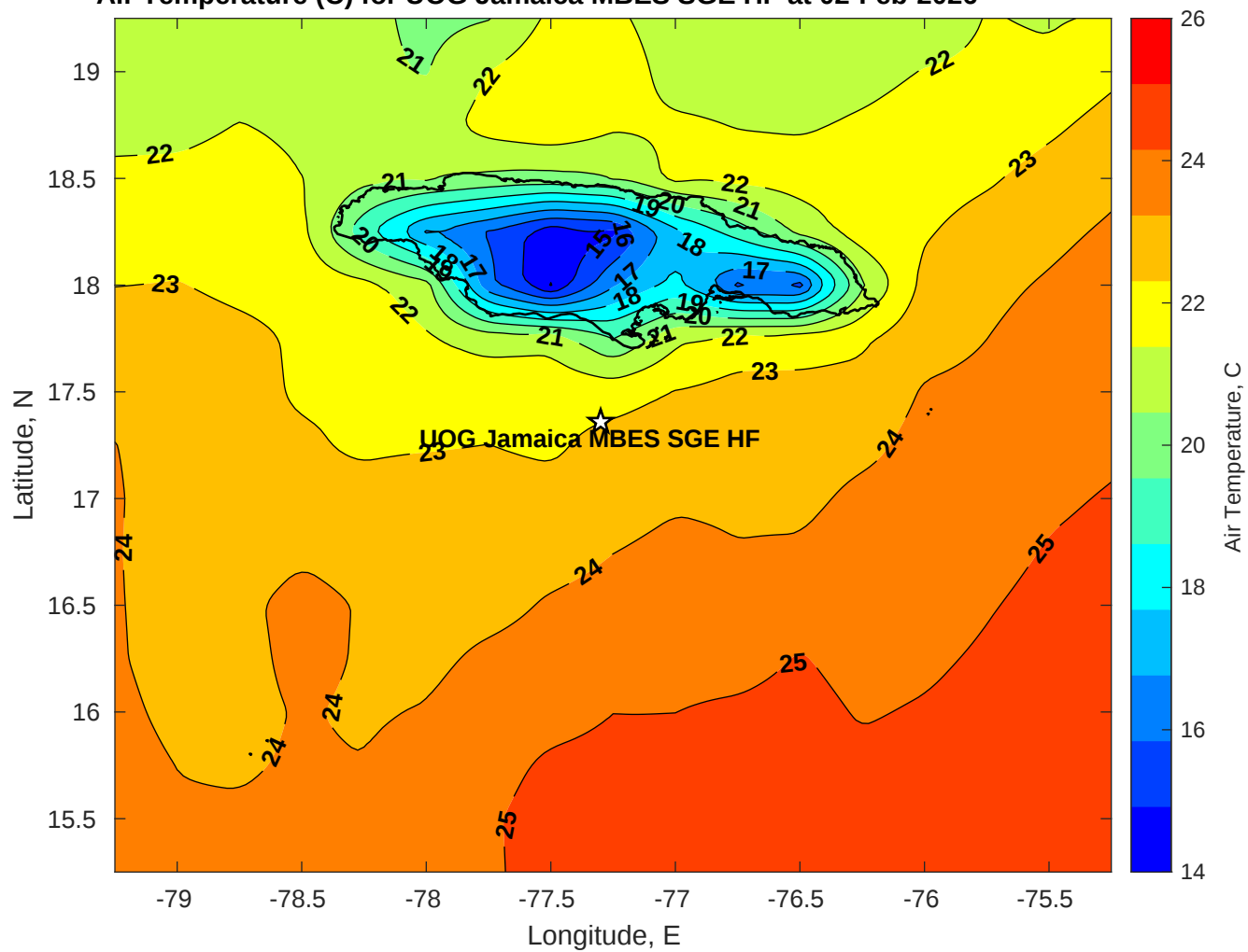
Air Temperature (C) for UOG Jamaica MBES SGE HF at 02-Feb-2026
