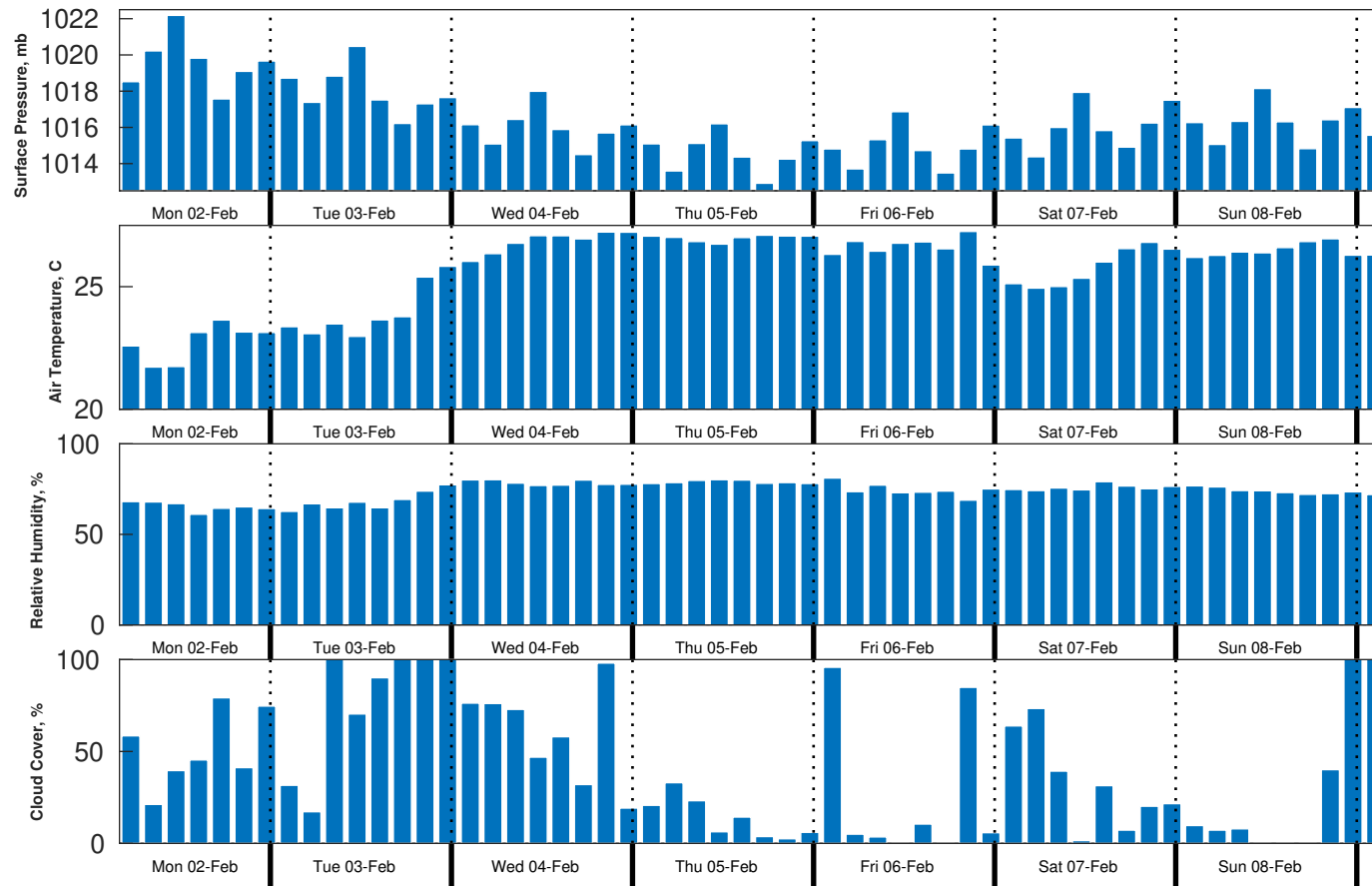
Met Forecast for UOG Jamaica MBES SGE HF from 02-Feb-2026 06:00:00 to 09-Feb-2026 06:00:00
