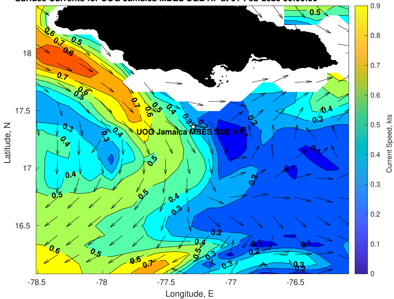
Surface Currents for UOG Jamaica MBES SGE HF at 01-Feb-2026 00:00:00
