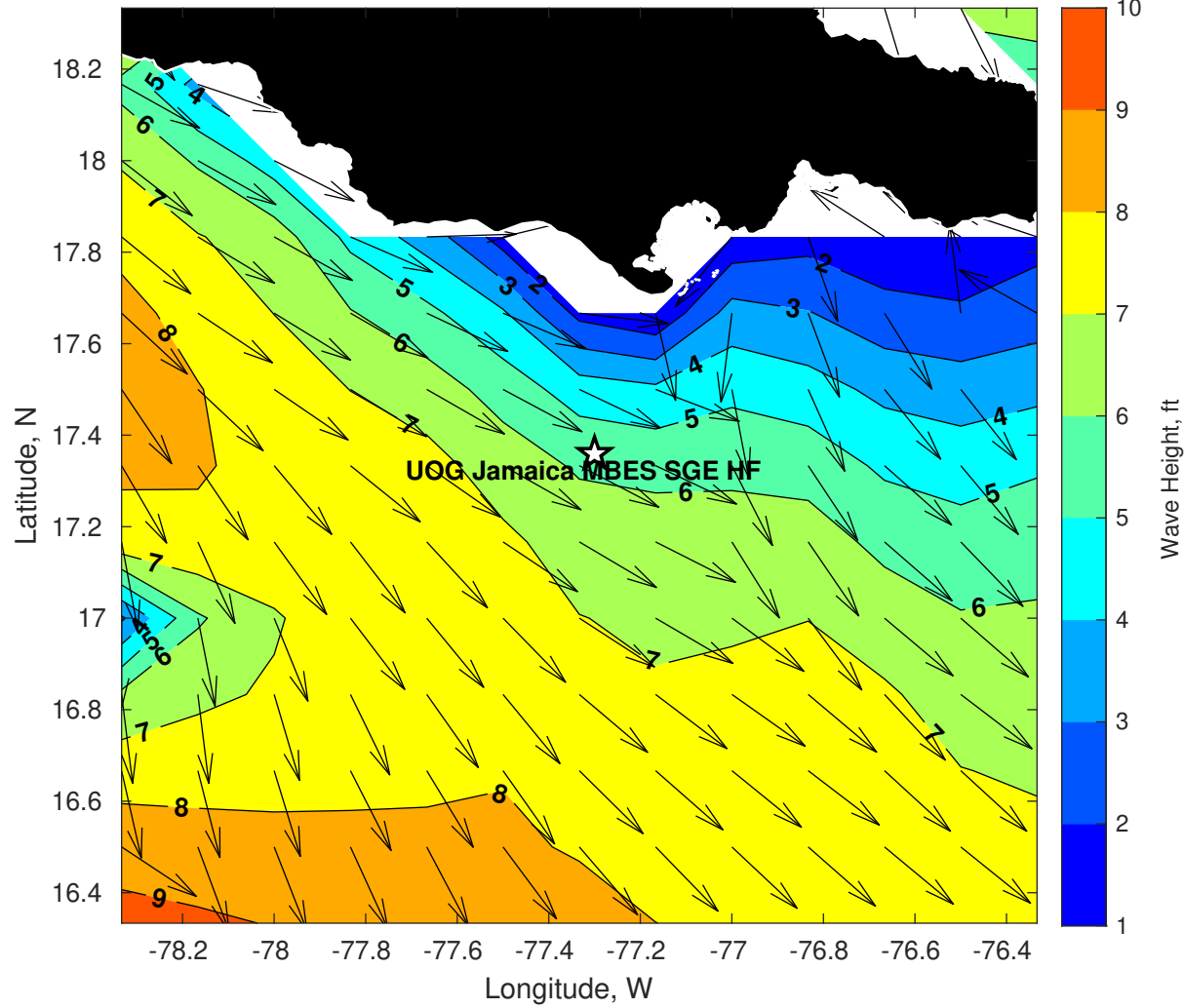
GFS Wave Height (ft) for UOG Jamaica MBES SGE HF at 02-Feb-2026 09:00:00
