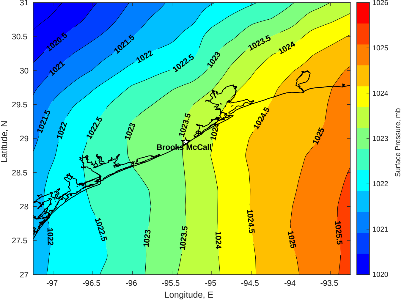
Surface Pressure (mb) for Brooks McCall at 03-Feb-2026 00:00:00
