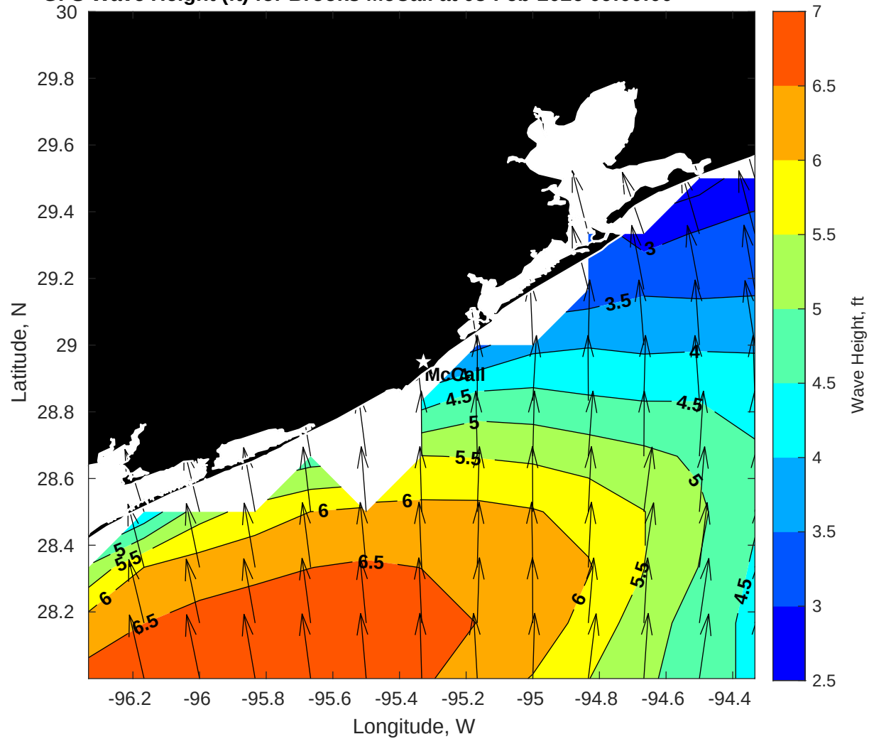
GFS Wave Height (ft) for Brooks McCall at 03-Feb-2026 09:00:00
