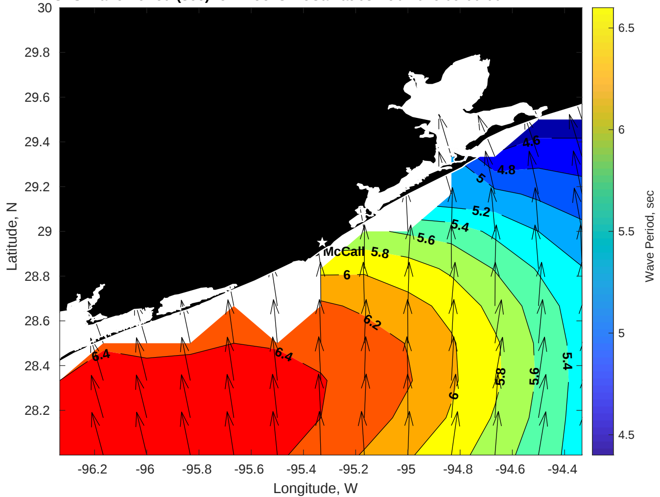
GFS Wave Period (sec) for Brooks McCall at 03-Feb-2026 09:00:00
