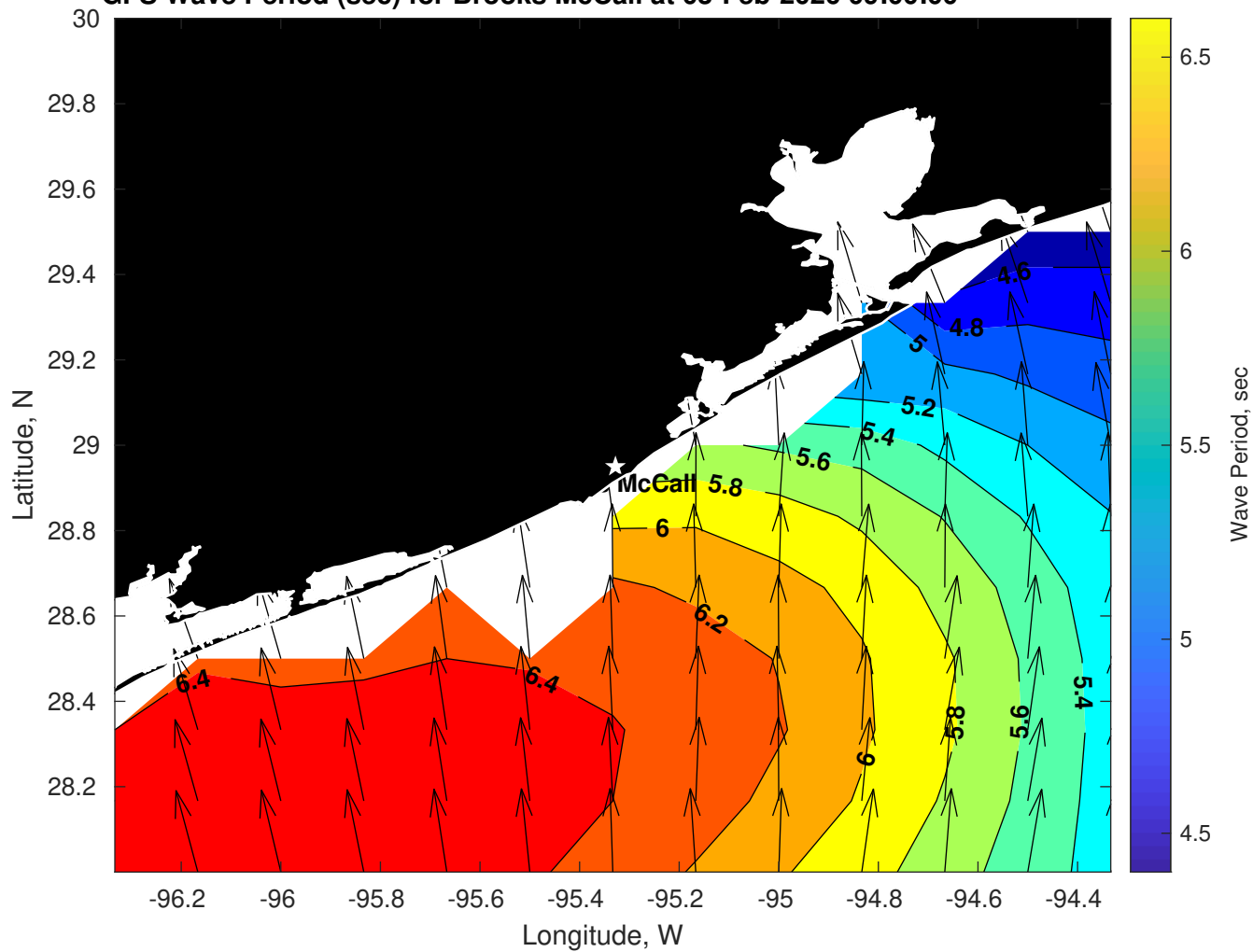
GFS Wave Period (sec) for Brooks McCall at 03-Feb-2026 09:00:00
