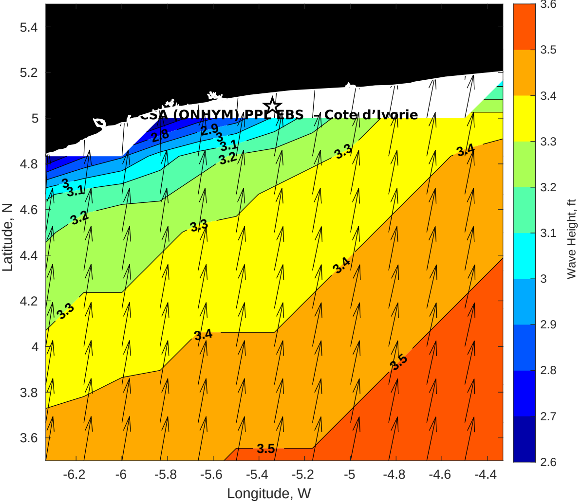
GFS Wave Height (ft) for CSA (ONHYM) PPL EBS - Cote d'Ivoire at 03-Feb-2026 09:00:00
