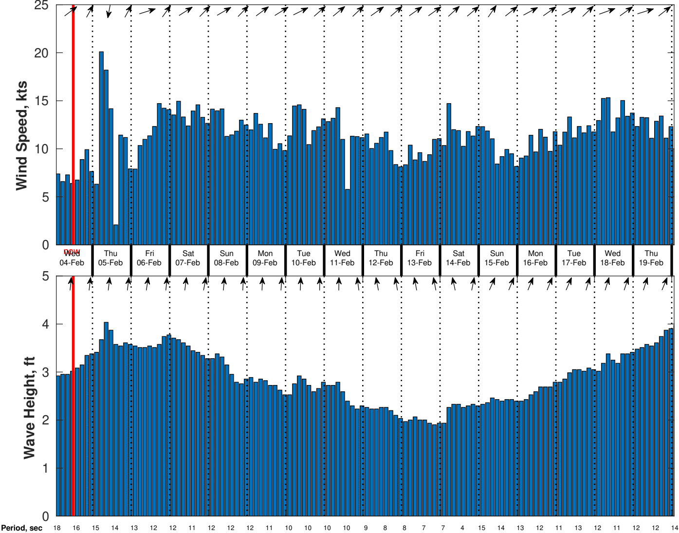
Wind & Wave Forecast for CSA (ONHYM) PPL EBS - Cote d'Ivoire from 03-Feb-2026 01:00:00 to 19-Feb-2026 01:00:00
