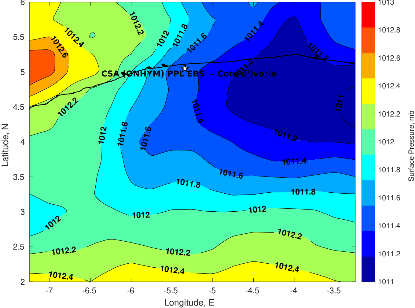
Surface Pressure (mb) for CSA (ONHYM) PPL EBS - Cote d'Ivoire at 05-Feb-2026 00:00:00
