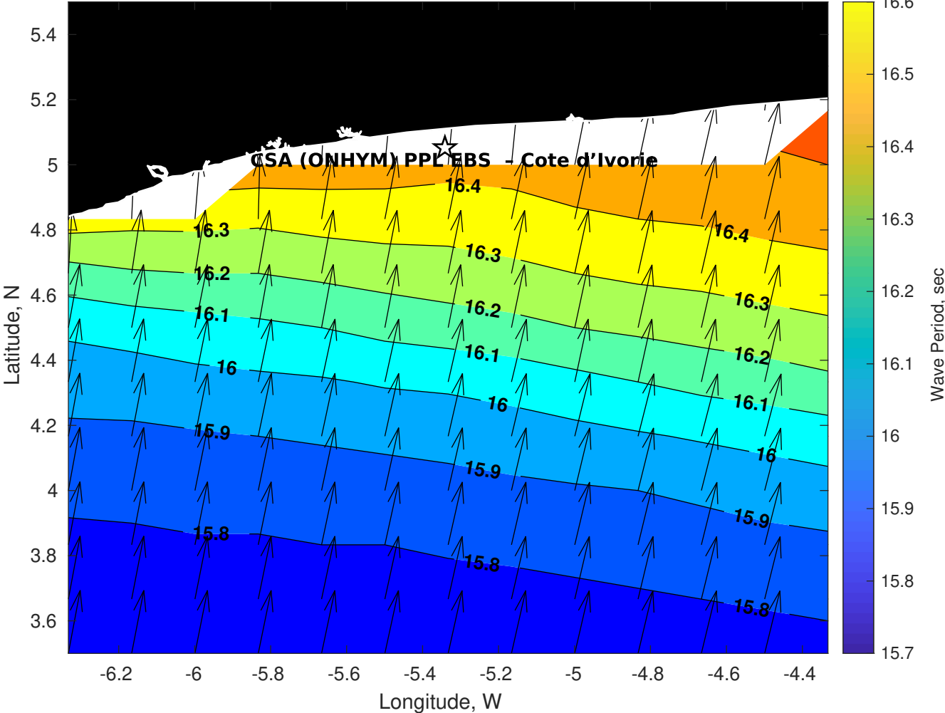
GFS Wave Period (sec) for CSA (ONHYM) PPL EBS - Cote d'Ivoire at 03-Feb-2026 09:00:00
