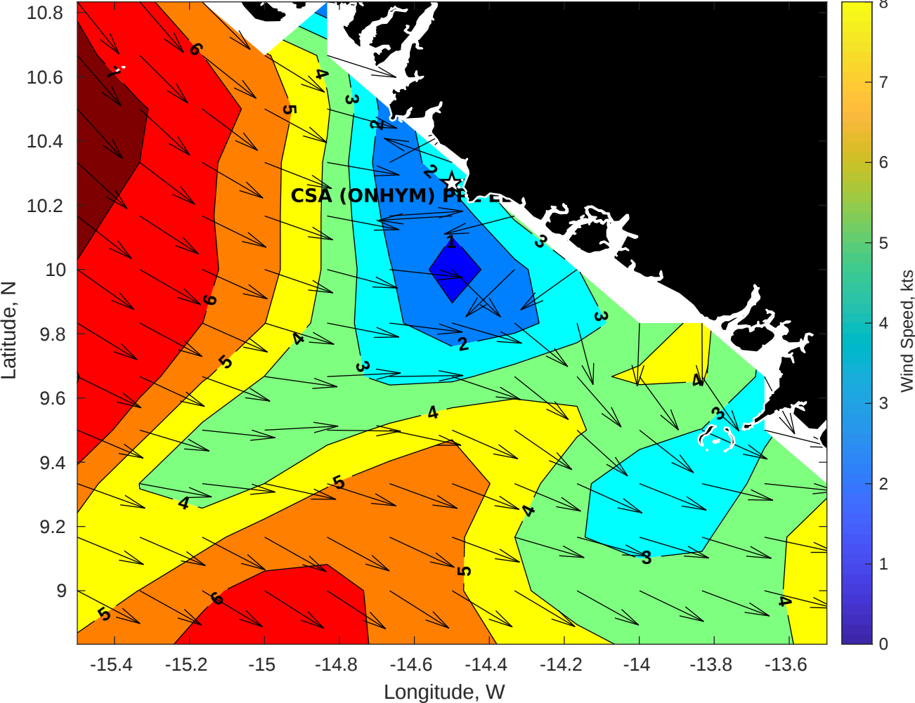
GFS Winds (kts) for CSA (ONHYM) PPL EBS - Guinea at 03-Feb-2026 09:00:00
