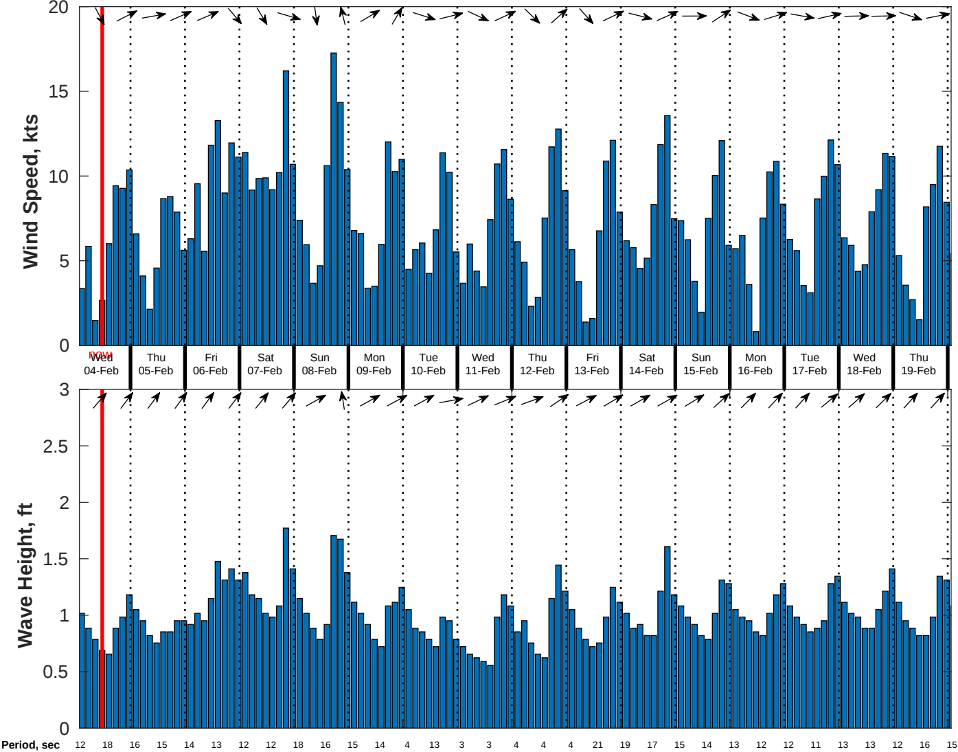
Wind & Wave Forecast for CSA (ONHYM) PPL EBS - Guinea from 03-Feb-2026 01:00:00 to 19-Feb-2026 01:00:00
