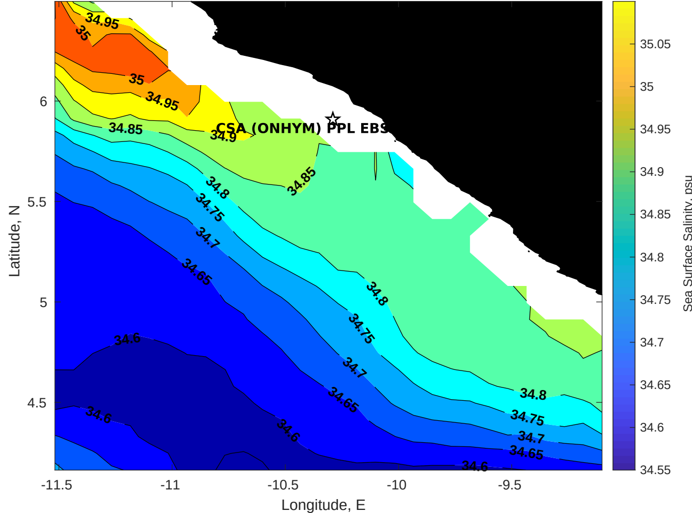
Surface Salinity for CSA (ONHYM) PPL EBS - Liberia at 02-Feb-2026 00:00:00
