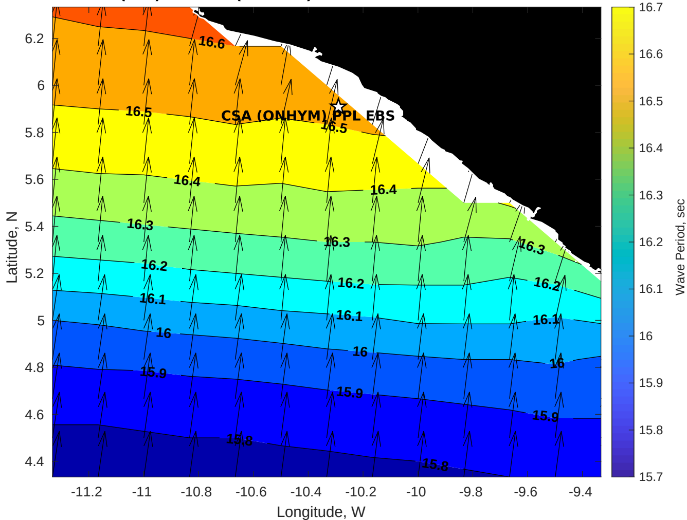
GFS Wave Period (sec) for CSA (ONHYM) PPL EBS - Liberia at 03-Feb-2026 09:00:00
