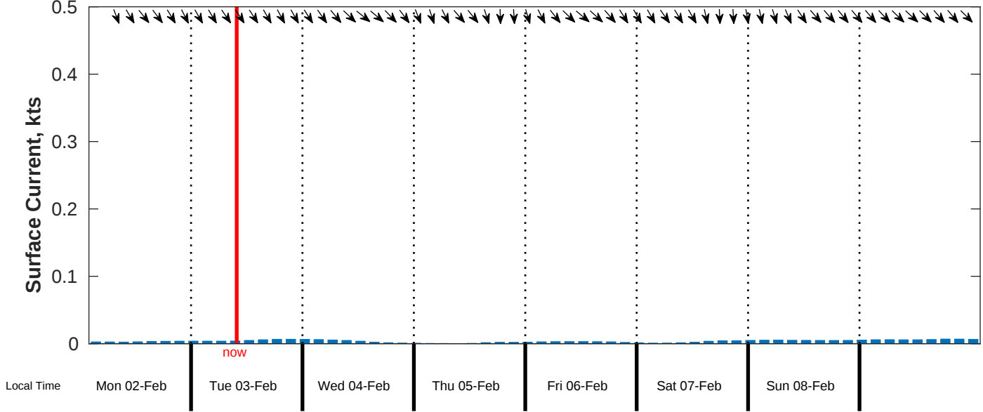
Surface Current Forecast for CSA (ONHYM) PPL EBS - Liberia from 02-Feb-2026 00:00:00 to 10-Feb-2026 00:00:00
