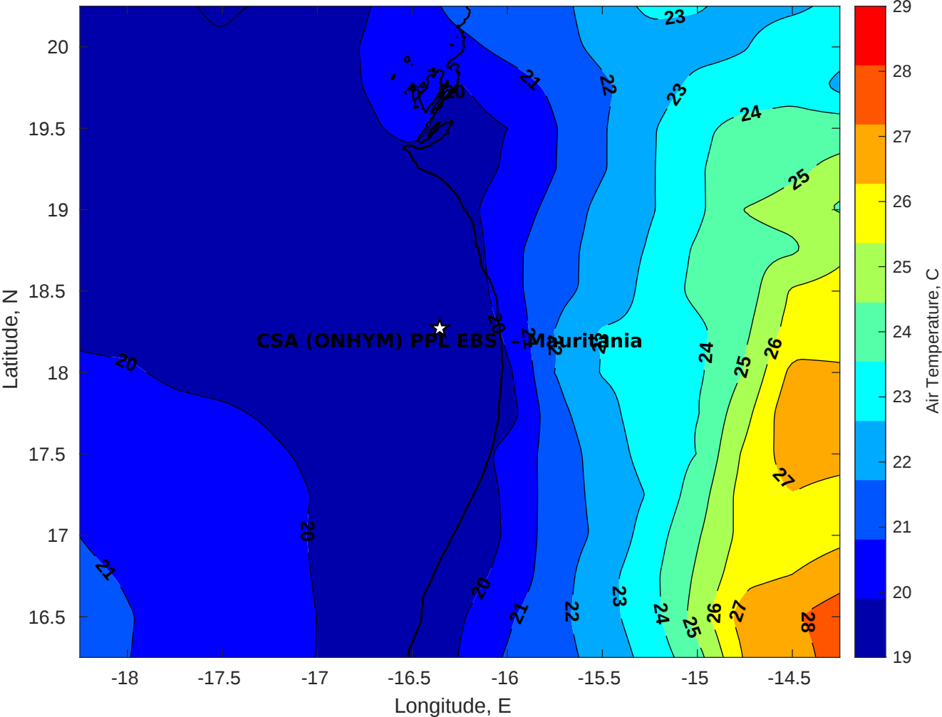
Air Temperature (C) for CSA (ONHYM) PPL EBS - Mauritania at 03-Feb-2026
