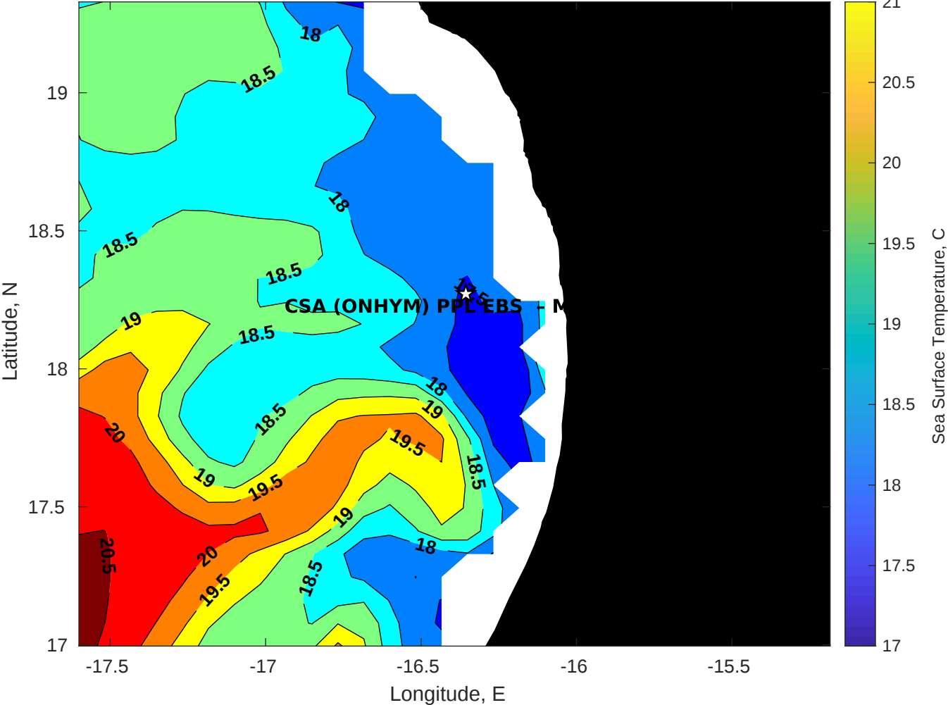
SST for CSA (ONHYM) PPL EBS - Mauritania at 02-Feb-2026 00:00:00
