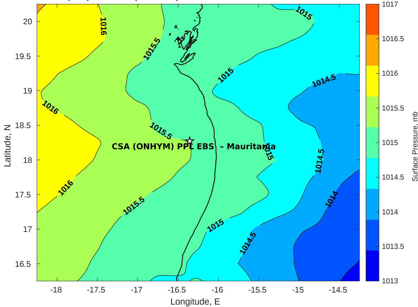
Surface Pressure (mb) for CSA (ONHYM) PPL EBS - Mauritania at 05-Feb-2026 00:00:00
