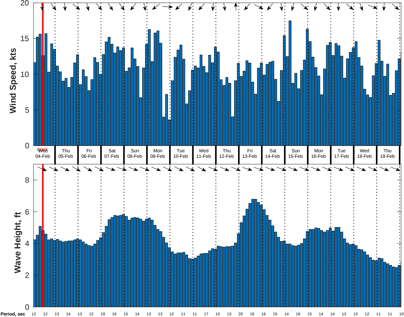
Wind & Wave Forecast for CSA (ONHYM) PPL EBS - Mauritania from 03-Feb-2026 01:00:00 to 19-Feb-2026 01:00:00
