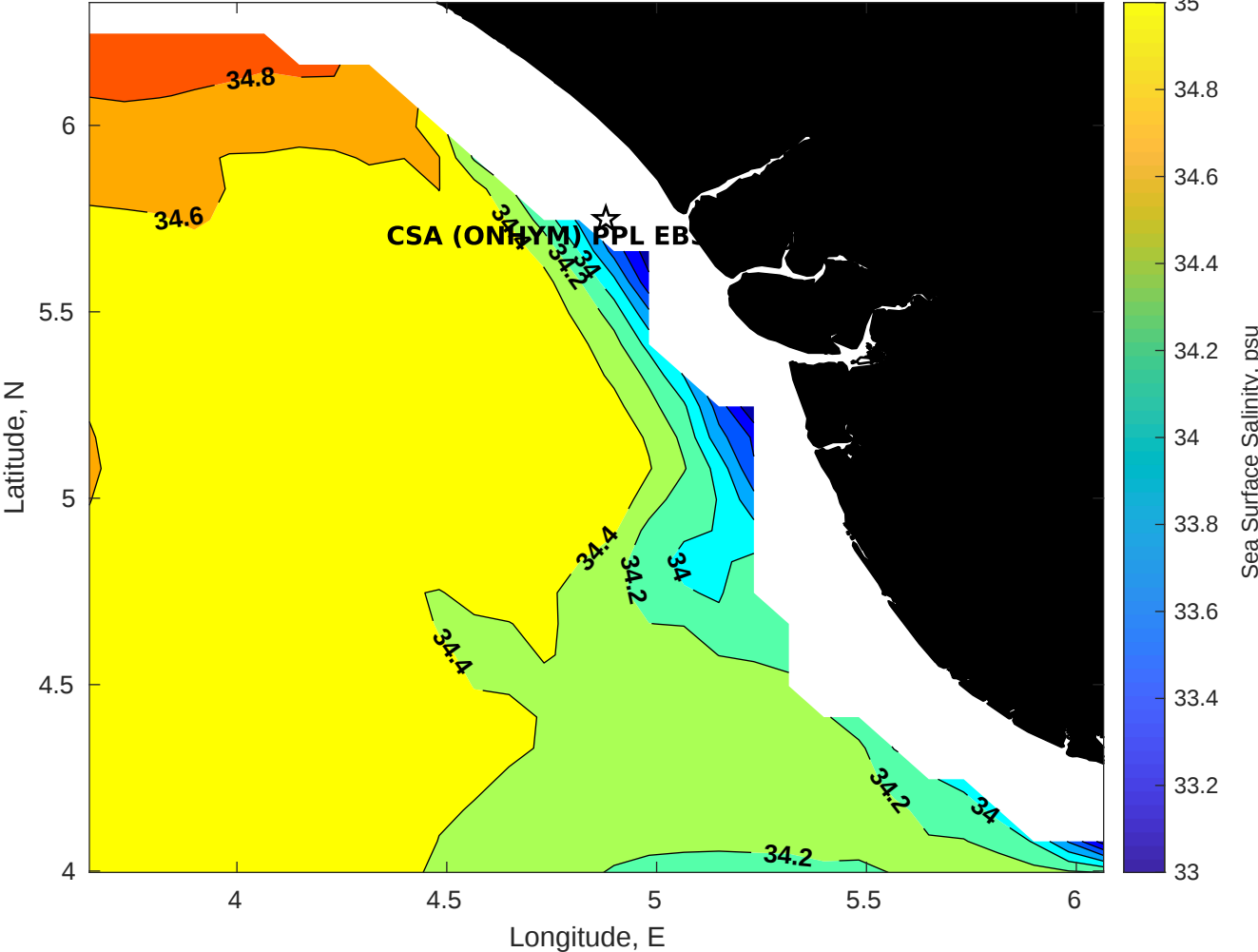
Surface Salinity for CSA (ONHYM) PPL EBS - Nigeria at 02-Feb-2026 00:00:00
