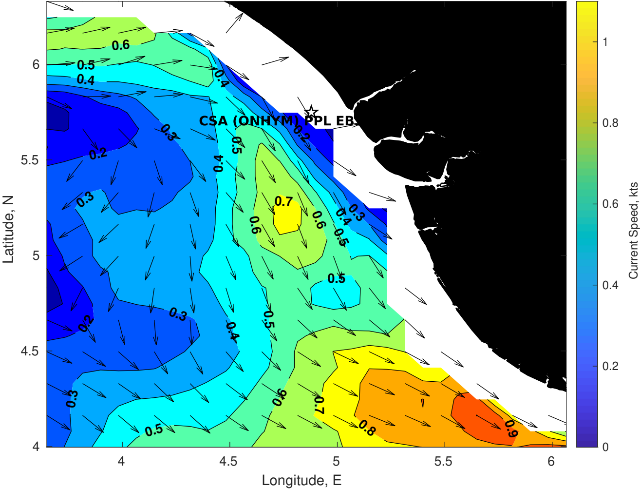
Surface Currents for CSA (ONHYM) PPL EBS - Nigeria at 02-Feb-2026 00:00:00
