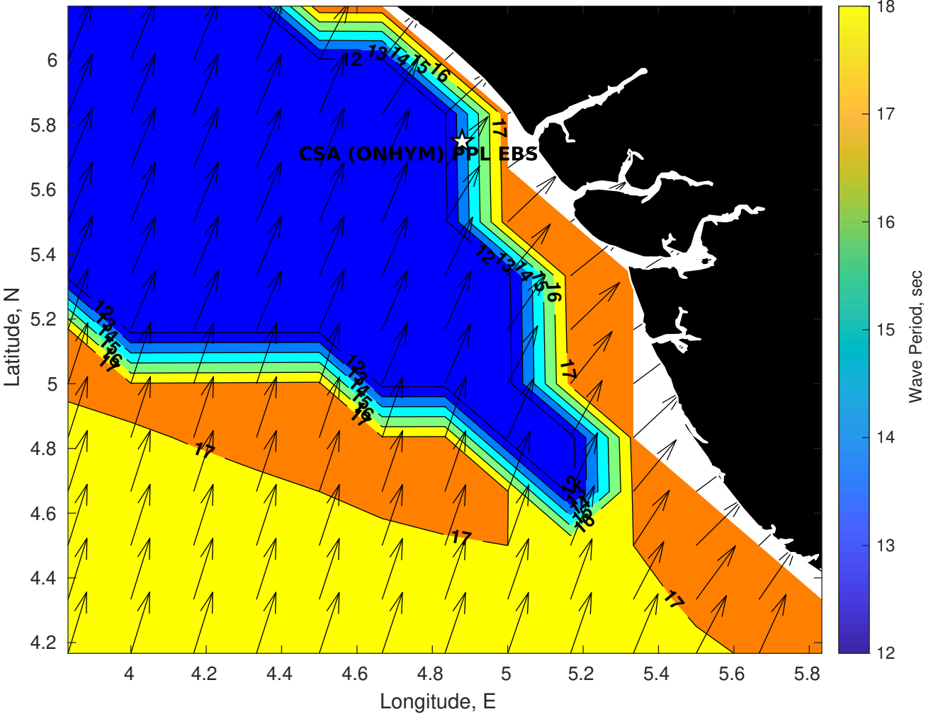
GFS Wave Period (sec) for CSA (ONHYM) PPL EBS - Nigeria at 03-Feb-2026 09:00:00
